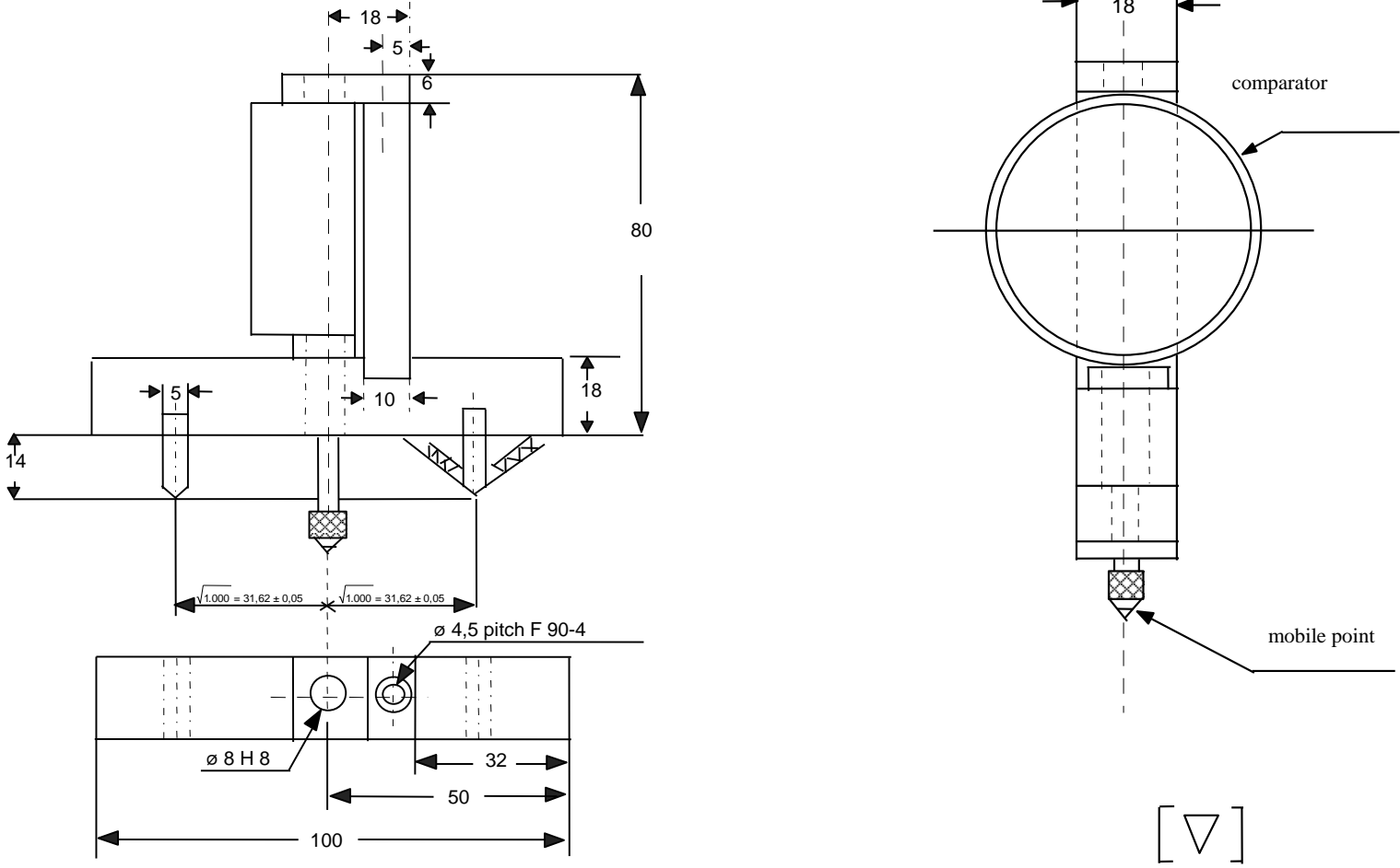
Figure 1 Spherometer
