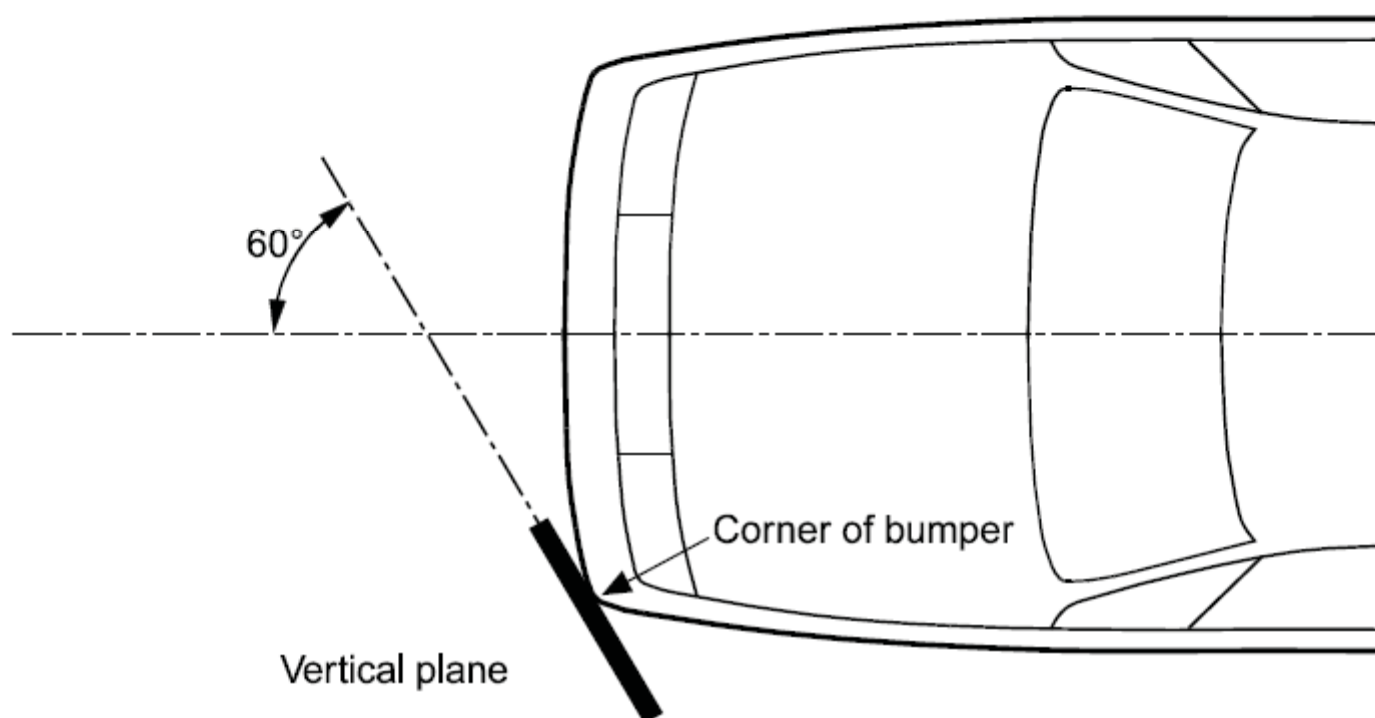
Figure 4: Determination of Bumper Corner
