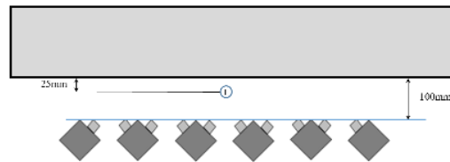
Figure 6k Position the Bottom of the Conformable Container Relative to the Burner
