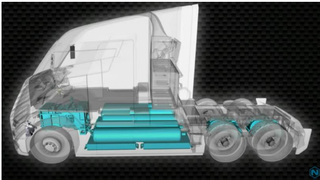
Example of a hydrogen fuel cell truck
