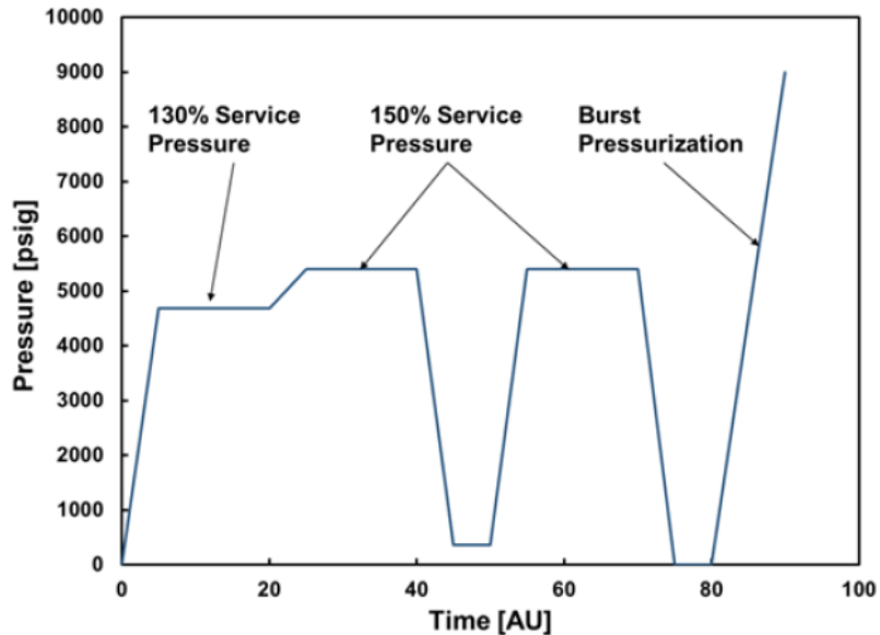
Figure 2. Pressure schedule for MAE examination followed by burst pressurization
