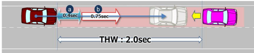
Figure 4 Deceleration scenario
