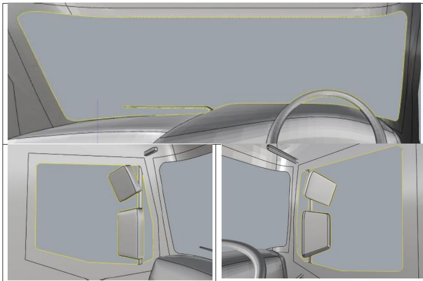
Figure 1345: Examples of drawing vision opening lines (yellow) for the frontal view (top), left view (left) and right view (right) in a CAD environment.
