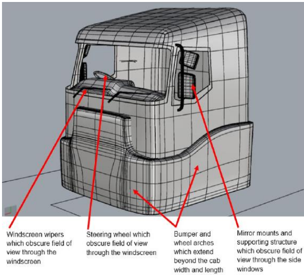
Figure 16: Illustration of the generic cab model
