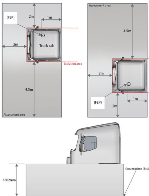
Figure 2: Definition of Assessment Volume
