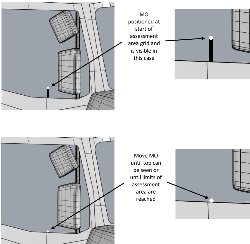
Figure 11. Positioning of MO to identify portions of gridlines in which the EH is visible
