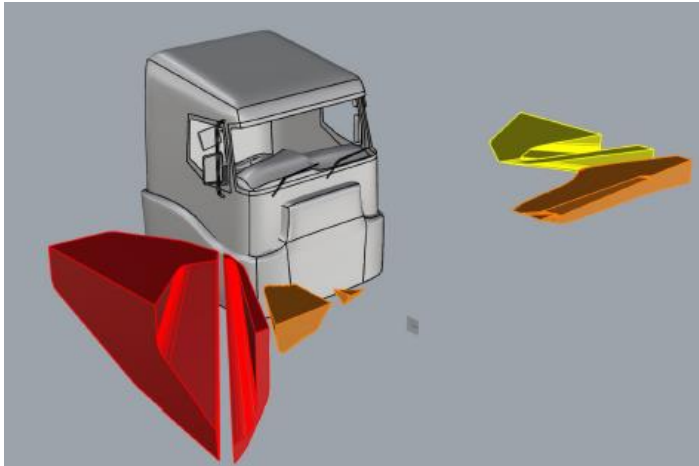
Figure 15: example of visible volume (RHD vehicle. Visible volume (nearside) yellow, front is orange, offside red)
