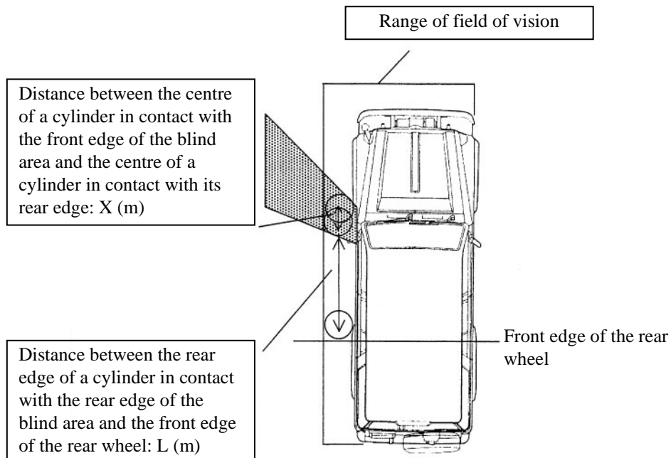
Figure B (right-handed drive case)
