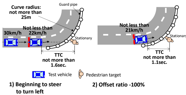
Figure 3: Curved road with guard pipes and a stationary object
