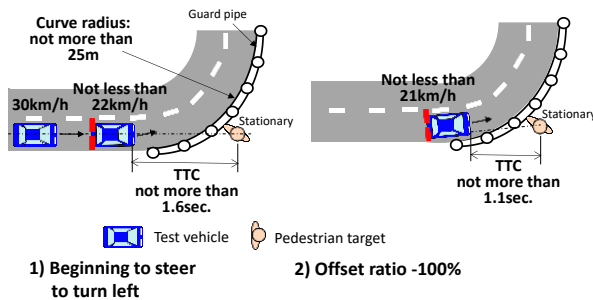
Figure 3: Curved road with guard pipes and a stationary object
