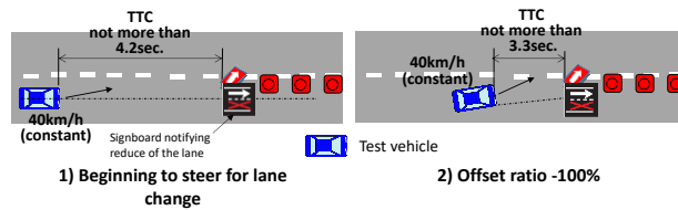
Figure 4: Lane change due to road construction
