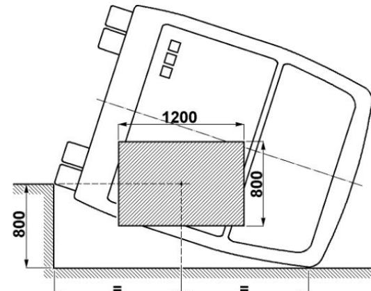
Figure A5.3a - Recommended field of view of outside camera
