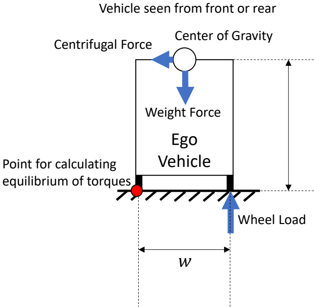
Figure 5: Lateral acceleration limit due to tipping
