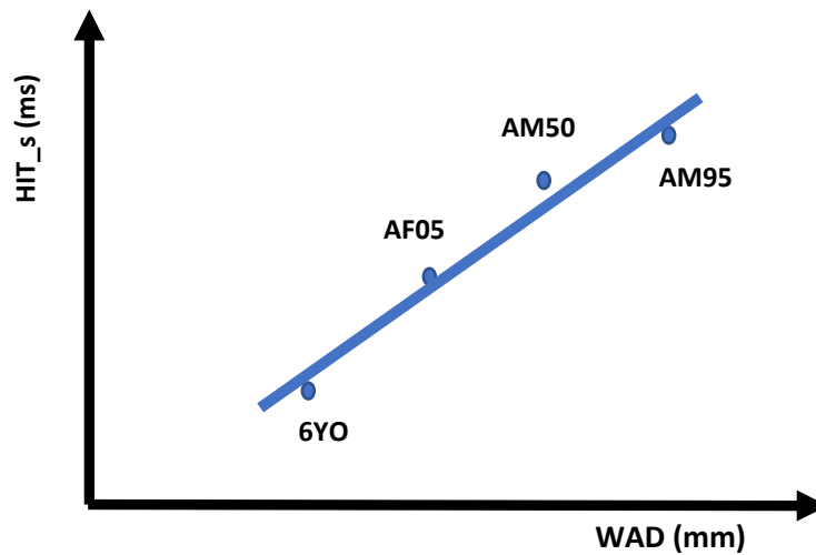
Head Impact Time(s for synchronisation) versus Wrap Around Distance (HIT_s vs WAD)
