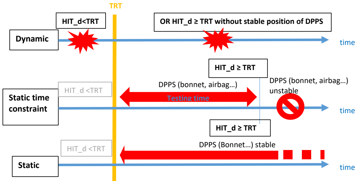
Figure 1-2 Timeline for dynamic, static time constraint and static testing representing real life conditions
