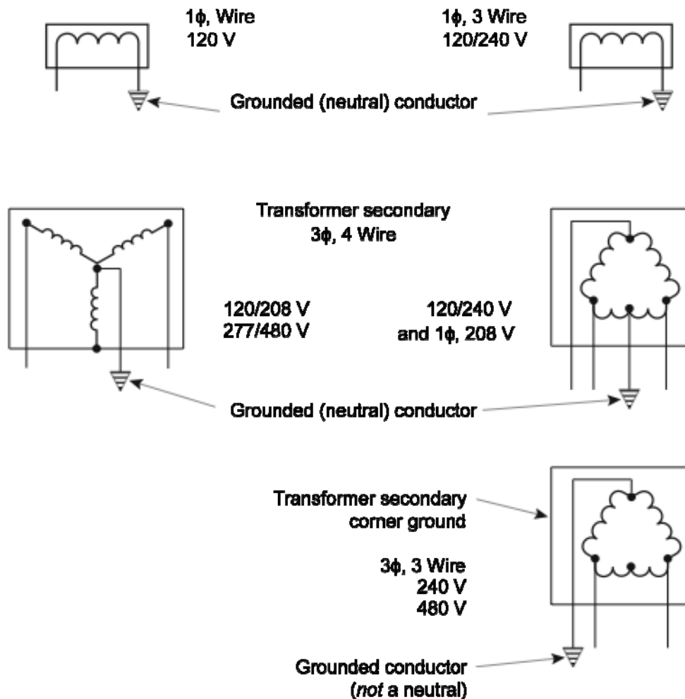
Fig. 5-5. Grounding for systems of 50 to 1,000 V AC.
