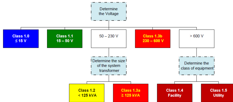
Fig. D-5. Hazard Classes 1.x, for 60 Hz Power.
