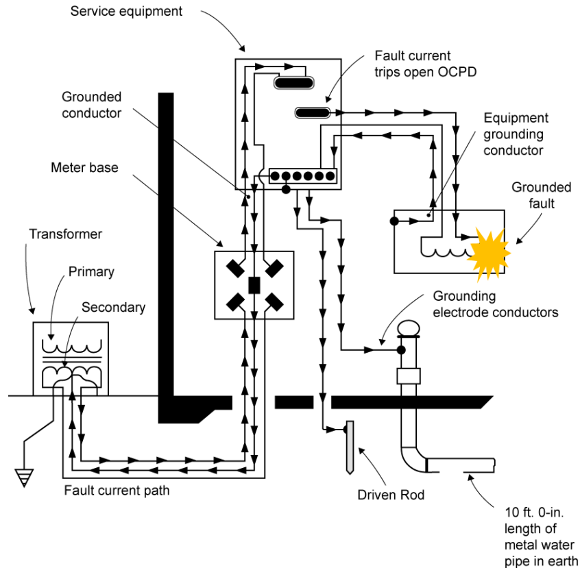
Fig. 5-6. The grounded neutral conductor.
