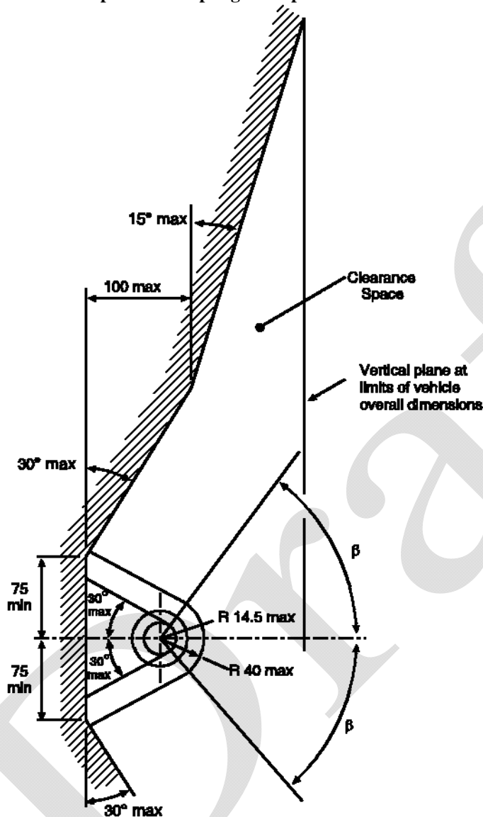
Figure 25 (b) Clearance space for coupling ball - plan view
