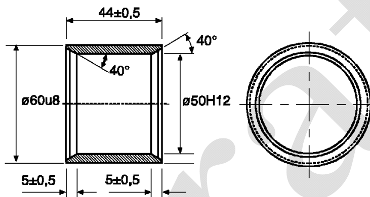
Figure 10 Non-slotted sleeve for Class D50-C drawbar eyes
