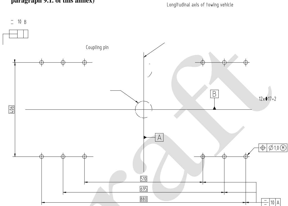
Figure 16a Mounting holes tolerances for class J mounting plates for fifth wheel couplings (see paragraph 9.1. of this annex)
