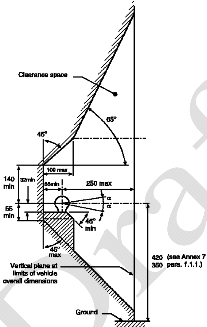
Figure 25 (a) Clearance space for, and height of, coupling ball - side view
