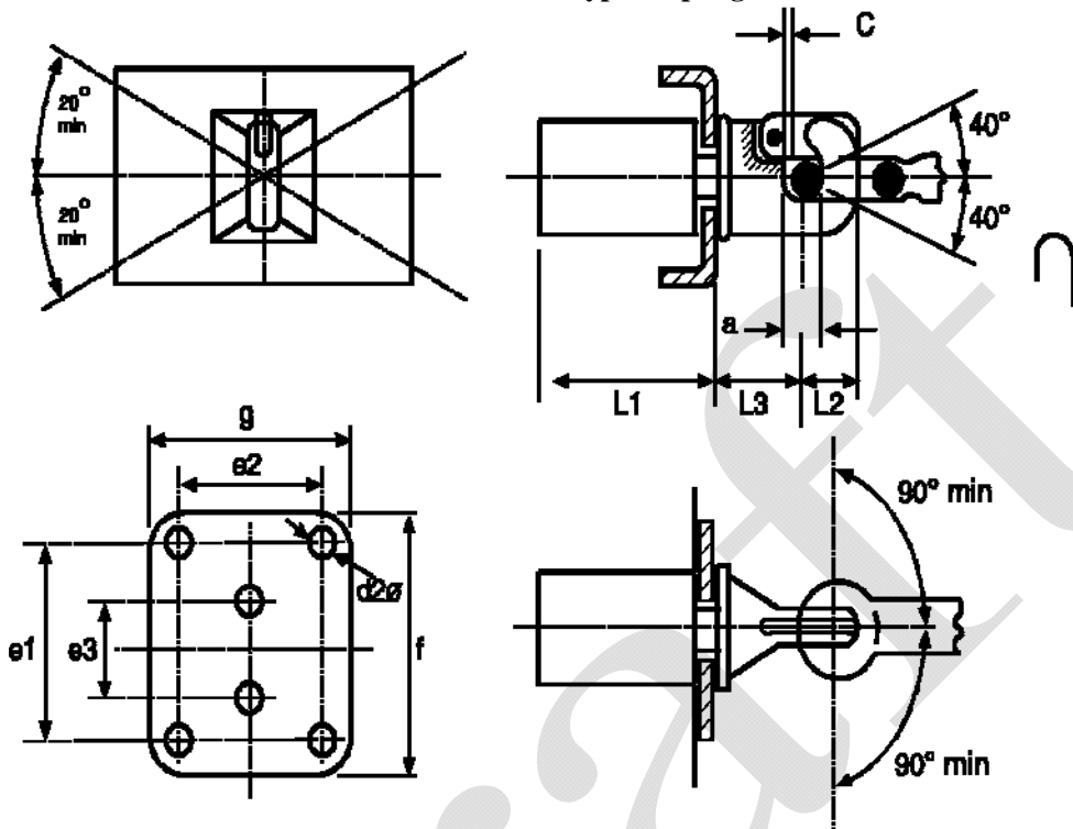
Figure 19 Dimensions and articulation of Class K hook type couplings
