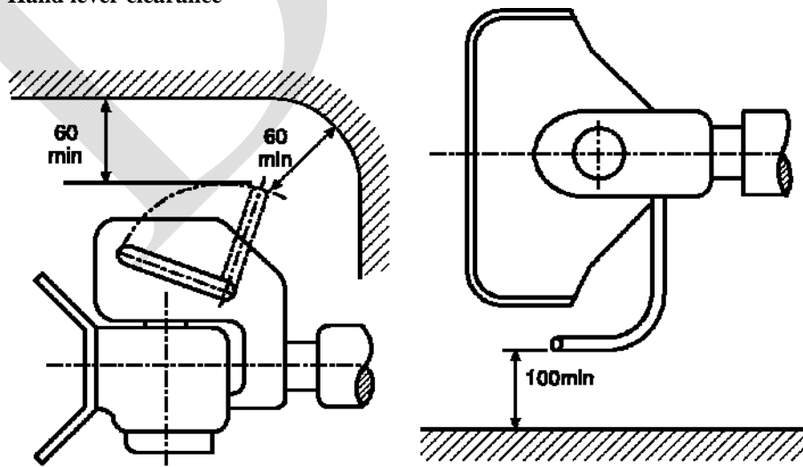
Figure 26 Hand lever clearance
