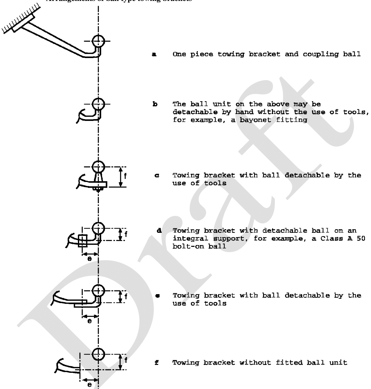
Figure 20 Arrangements of ball type towing brackets
