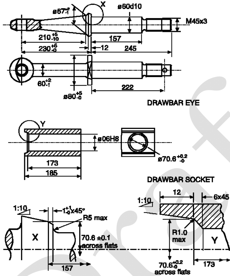
Figure 12 Dimensions of Class D50-B drawbar eyes, see other dimensions in Figure 11
