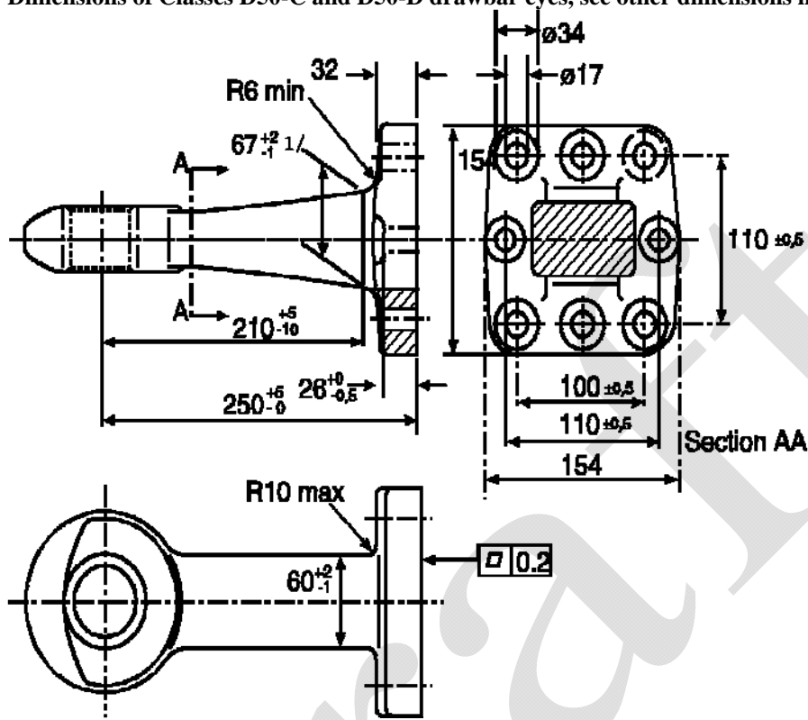
Figure 13 Dimensions of Classes D50-C and D50-D drawbar eyes, see other dimensions in Figure 11
