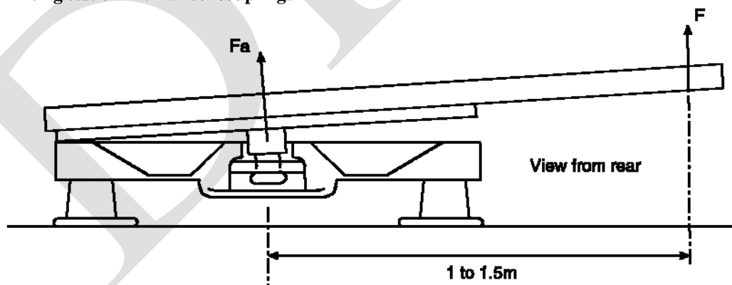
Figure 24 Lifting test on fifth wheel couplings
