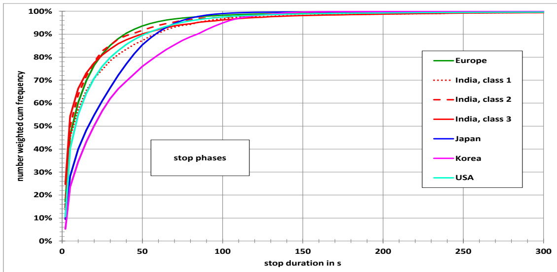
Figure 2: Stop duration distributions (number weighted) for different regions
