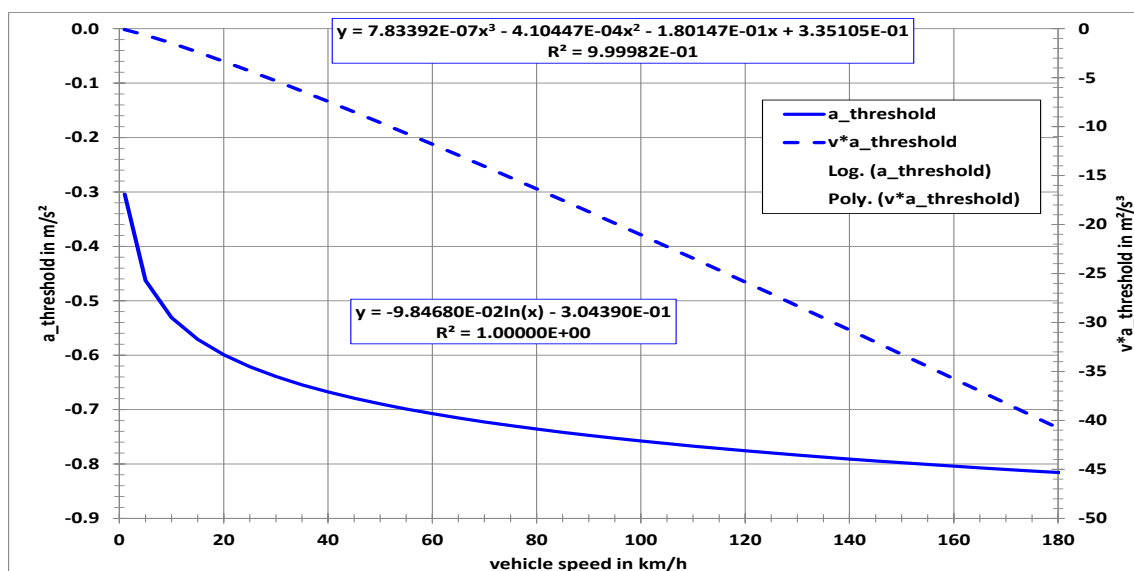
Figure 15: Threshold curves for the determination of brake engagement phases
