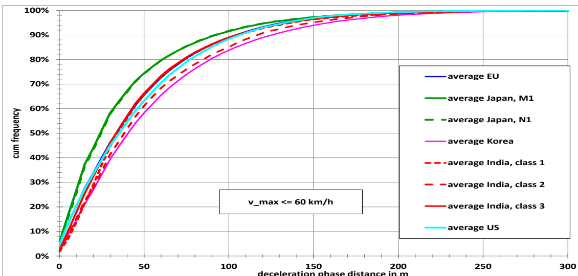
Figure 13a: Deceleration phase duration distributions for the different regions and max speed \leq 60 km/h
