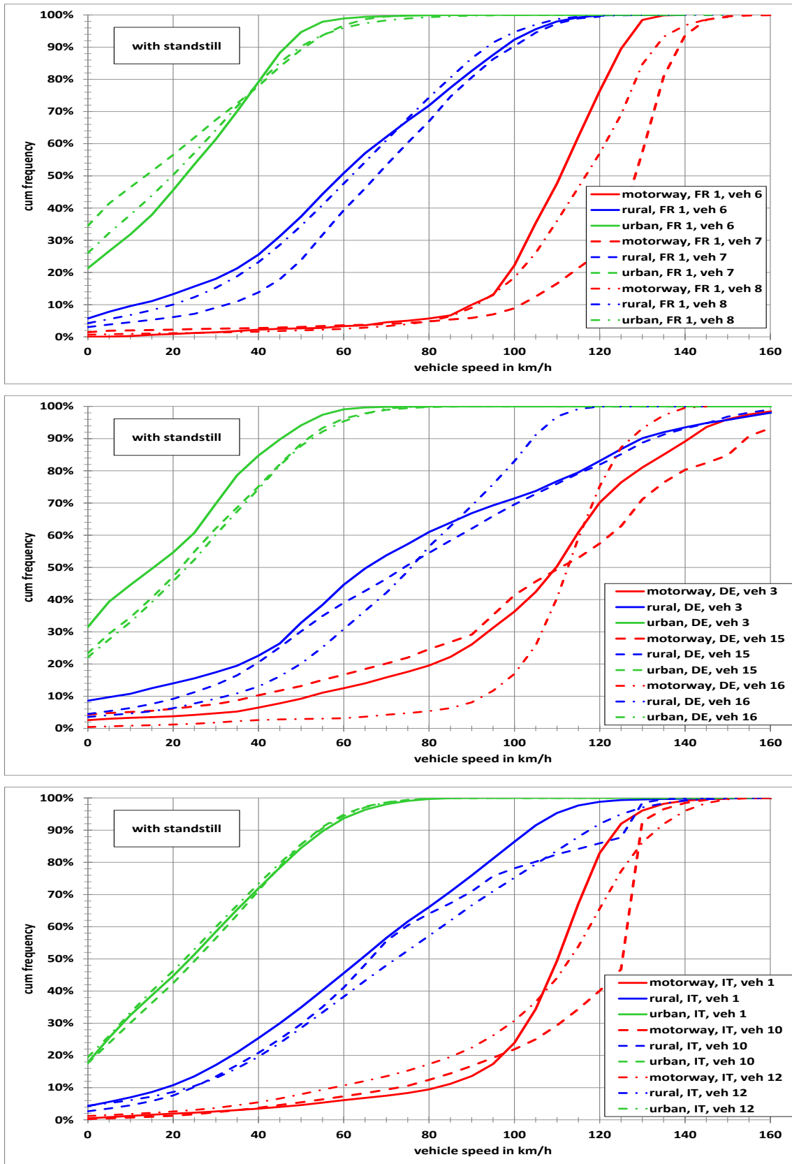
Figure 2: Vehicle speed distributions for different road categories in the European campaign: a (France), b (Germany), and c (Italy)
