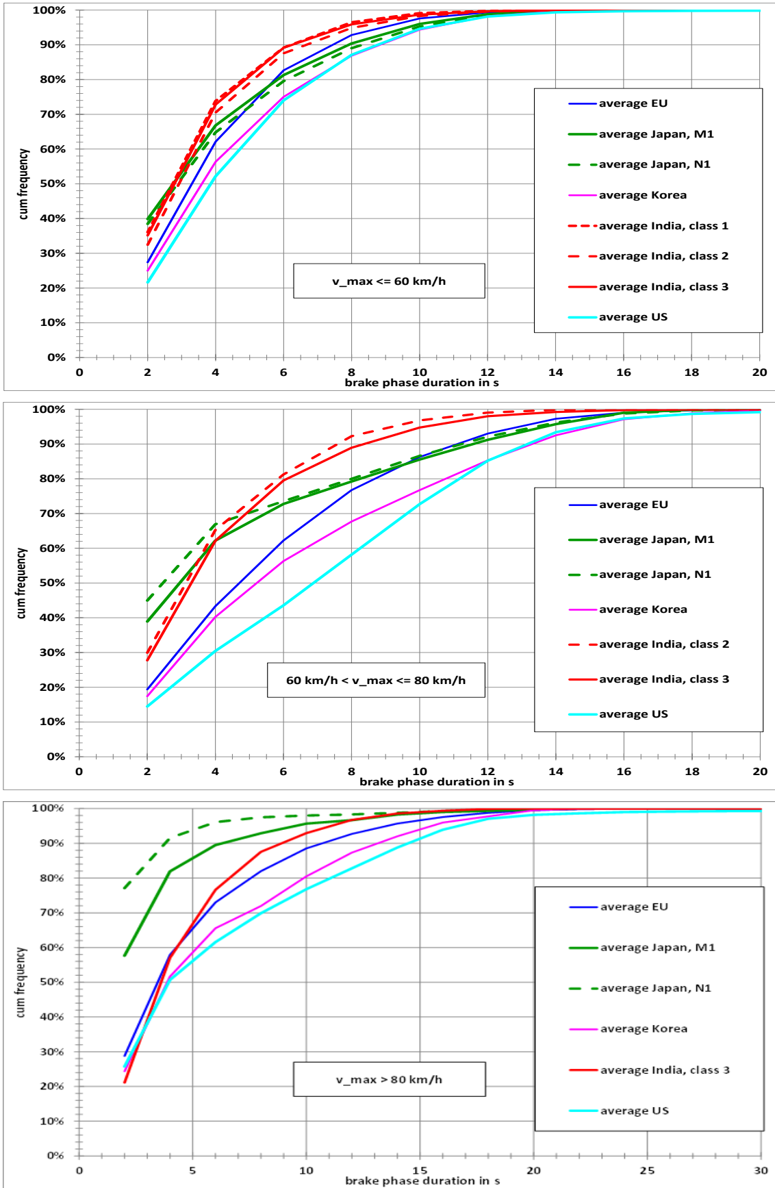
Figure 36: Brake phase duration distributions for the different regions and maximum speed categories: a. (max speed \leq 60 \text{ km/h} ), b. ( 60 \text{ km/h} < \text{max speed} \leq 80 \text{ km/h} ), c. (max speed > 80 \text{ km/h} )
