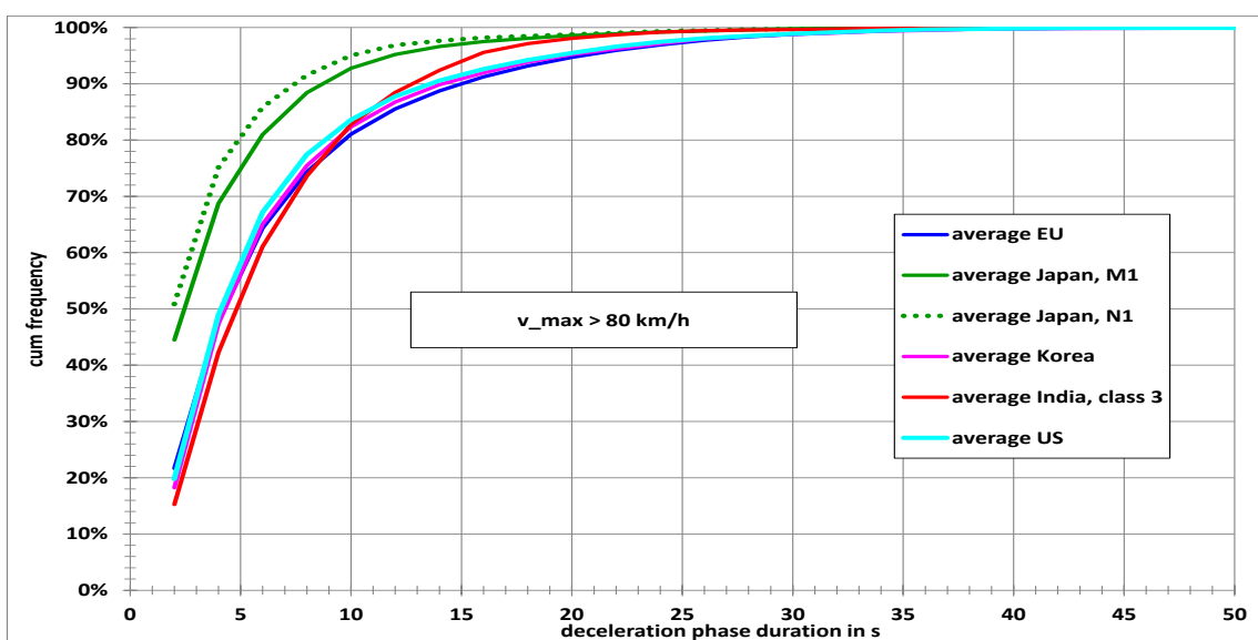
Figure 11: Deceleration phase duration distributions for the different regions and different max speeds: a ( \leq 60 km/h), b ( 60 \text{ km/h} < \text{max speed} \leq 80 \text{ km/h} ), and c ( > 80 \text{ km/h} )
