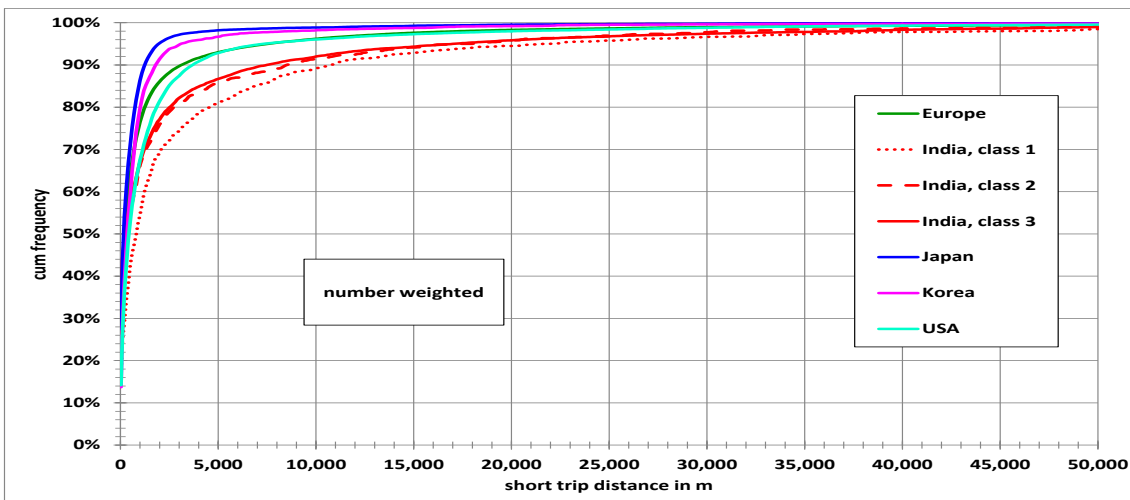
Figure 5: Short trip distance distributions (number weighted) for different regions
