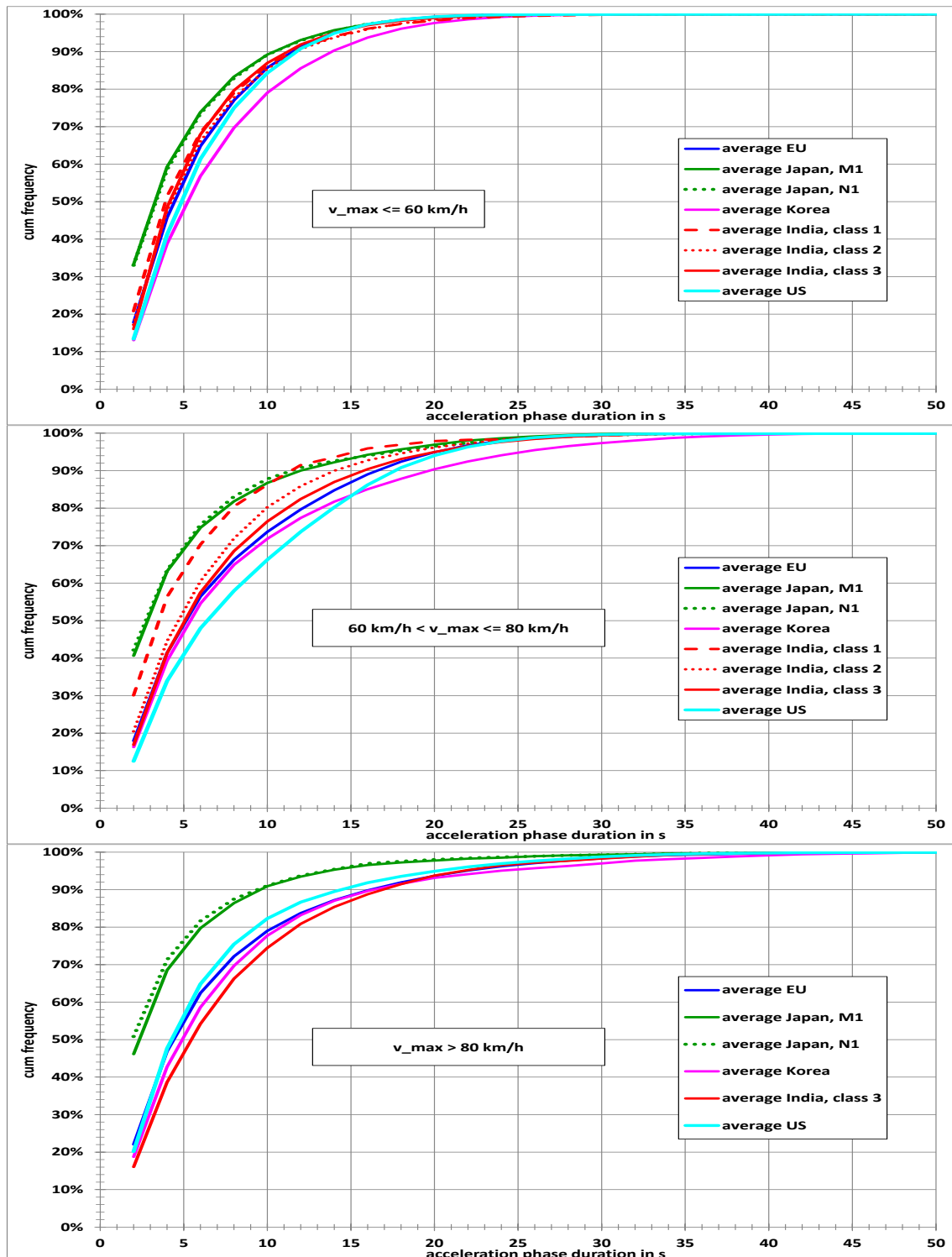
Figure 7: Acceleration phase duration distributions [s] for different maximum speed category worldwide: a. ( \leq 60 km/h), b. ( 60 km/h < max speed \leq 80 km/h), and c. ( > 80 km/h)
