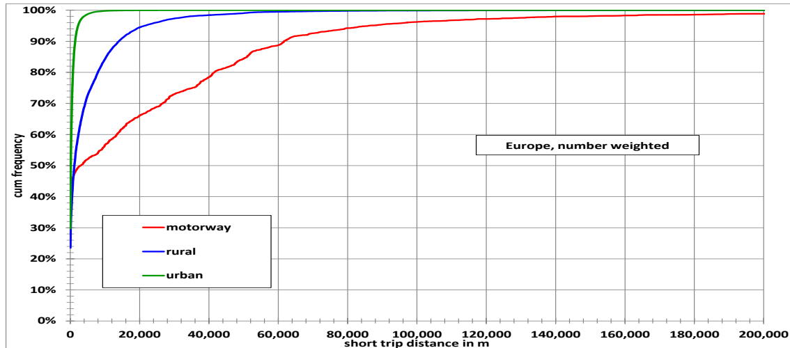
Figure 6: Short trip distance distributions for Europe separated for road categories
