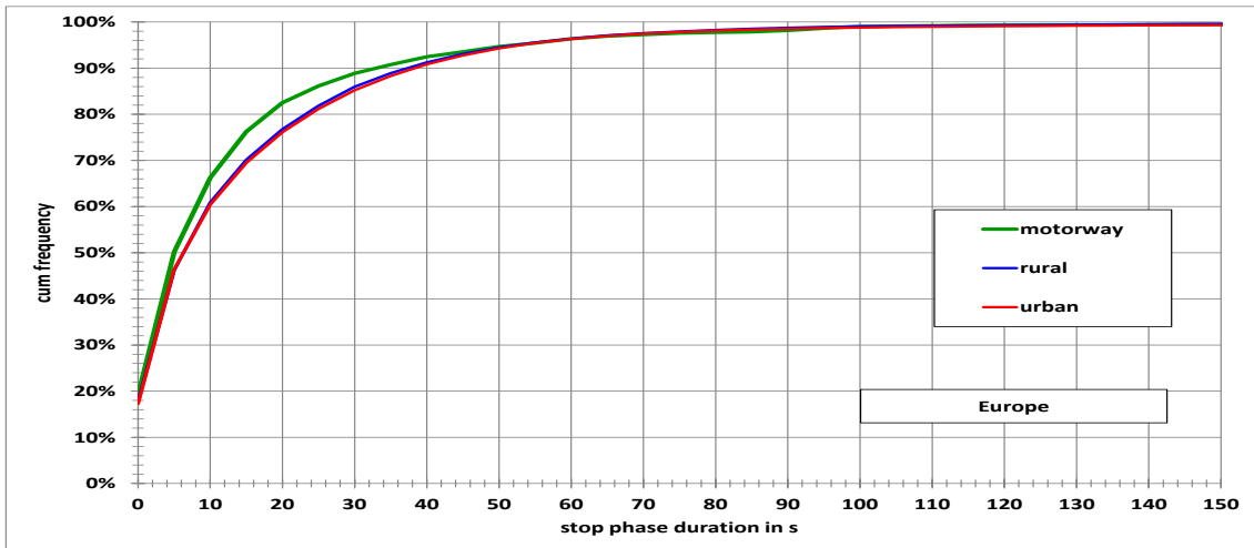
Figure 4: Stop duration distributions (number weighted) for different road categories
