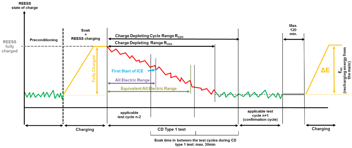
Figure A8.App1/1 OVC-HEVs, charge-depleting Type 1 test
