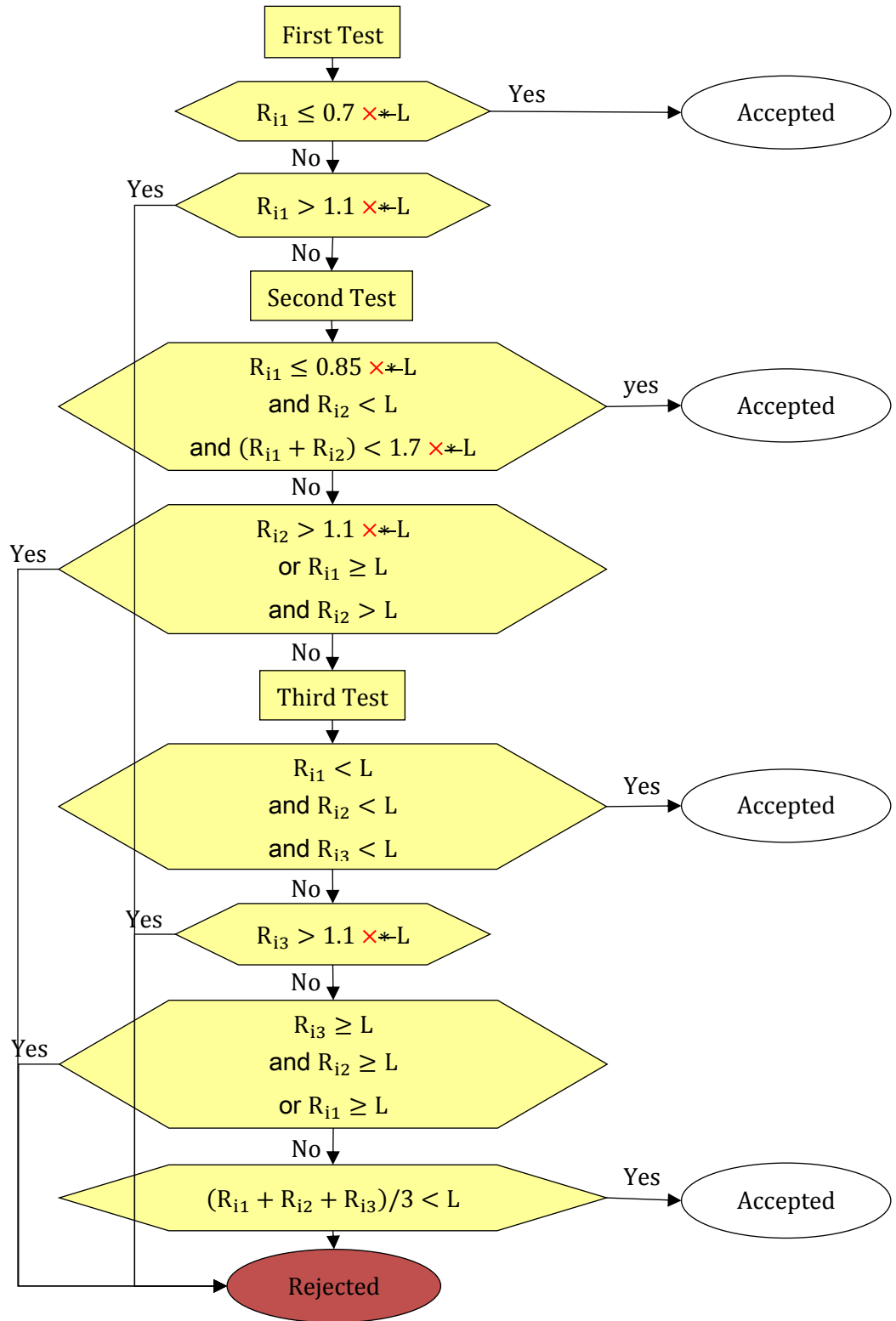
Figure A6/1 Flowchart for the nNumber of Type 1 tests
