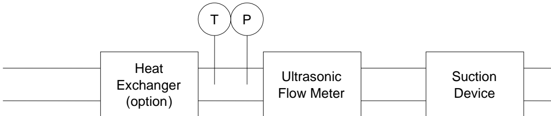
Schematic of an ultrasonic flow meter (UFM USM )
