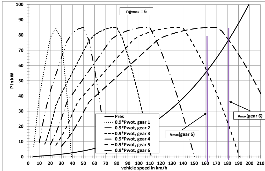
Figure 1a An example where ng_{\max} is the highest gear
