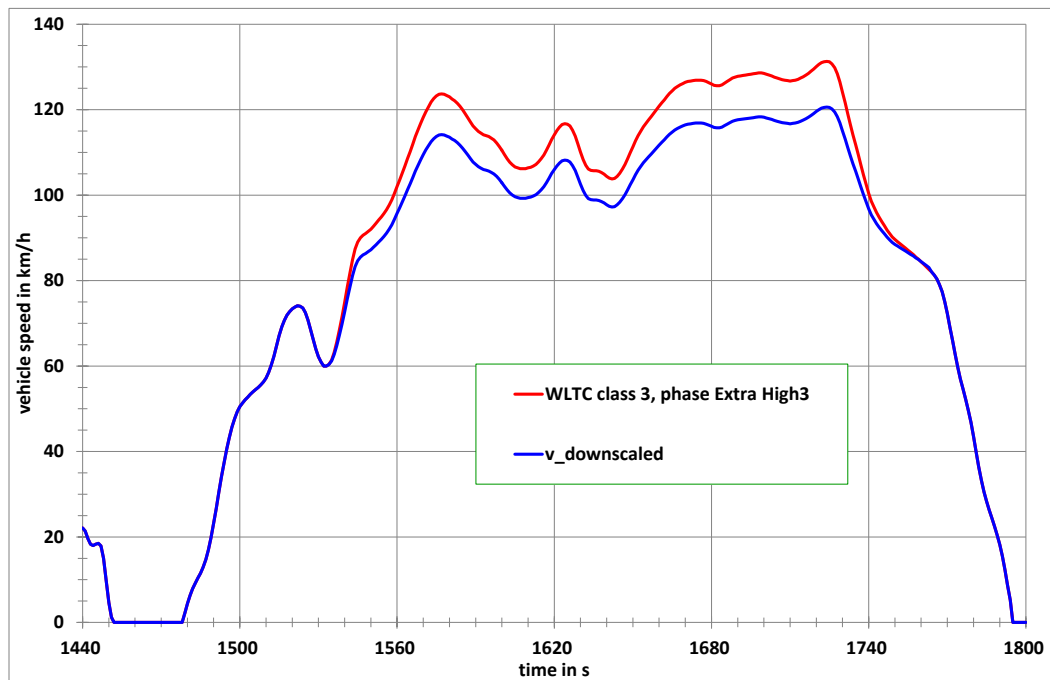
Figure A1/45-16 Downscaled extra high speed phase of the Class 3 WLTC
