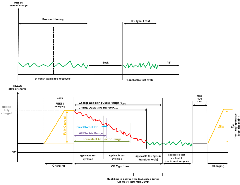
Figure A8.App1/4 OVC-HEVs, charge-depleting Type 1 test with subsequent charge-sustaining Type 1 test
