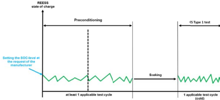
Figure A8.App1/2 OVC-HEVs, charge-sustaining Type 1 test
