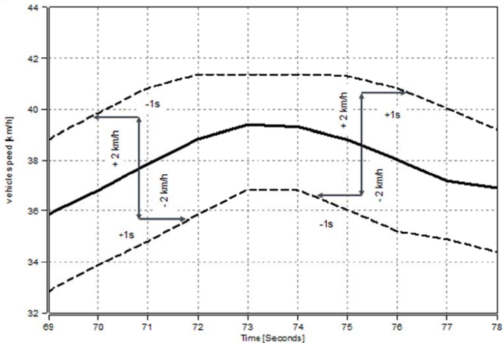
Figure A6/2 Speed trace tolerances
