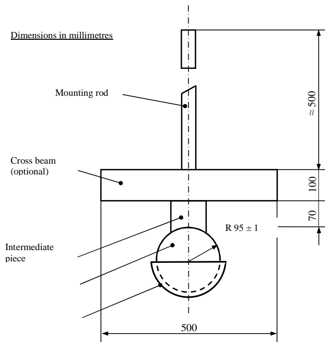
Figure 2: Head-form
