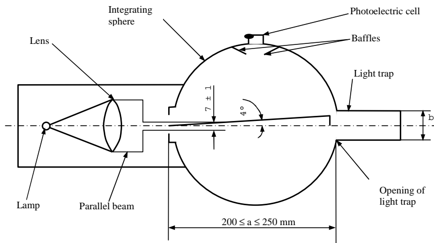
Figure 5: Hazemeter
