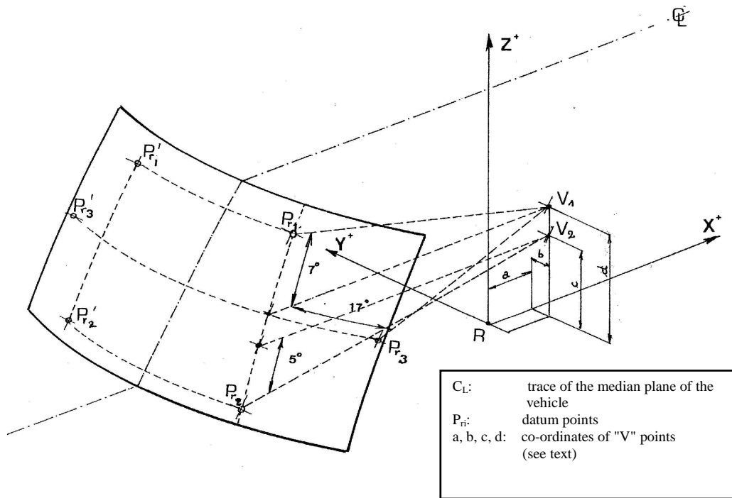
Figure 3: Determination of the datum points
