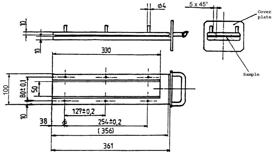
Figure 17: Example of sample holder
