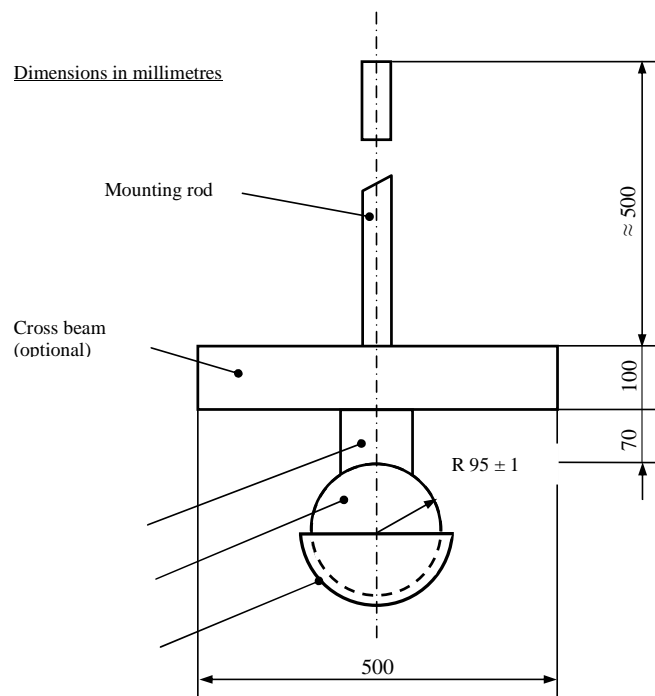
Figure 2: Head-form
