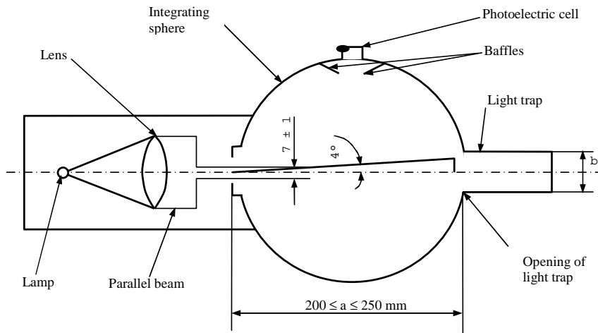
Figure 5: Hazemeter
