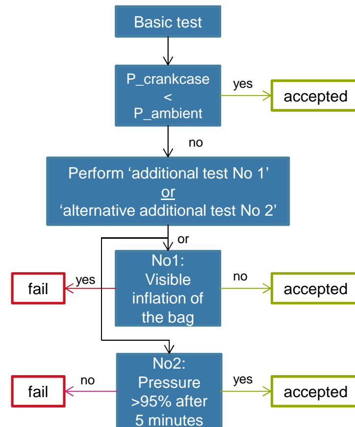
Type III: Crankcase emissions
