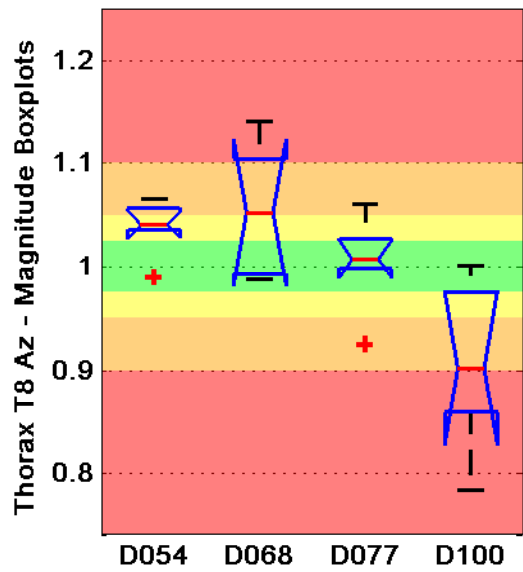
Taxicab Norm
