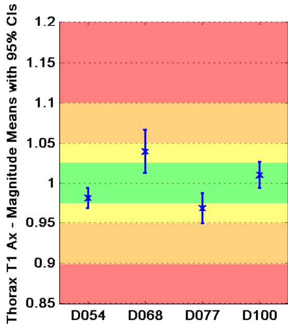
Taxicab Norm
