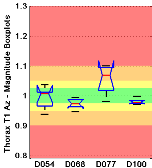
Taxicab Norm
