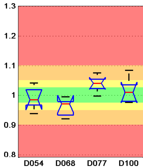
Euclidian Norm
