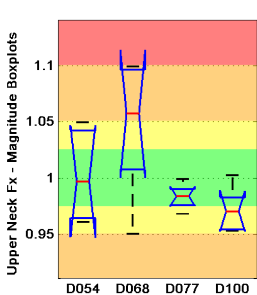
Taxicab Norm
