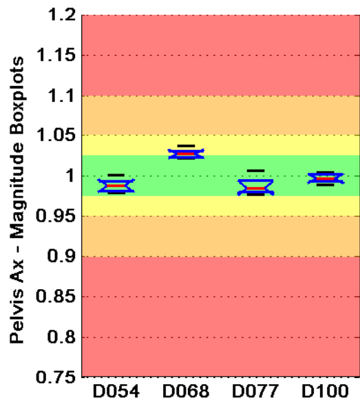
Taxicab Norm
