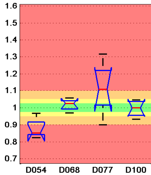
Euclidian Norm
