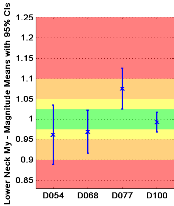
Taxicab Norm
