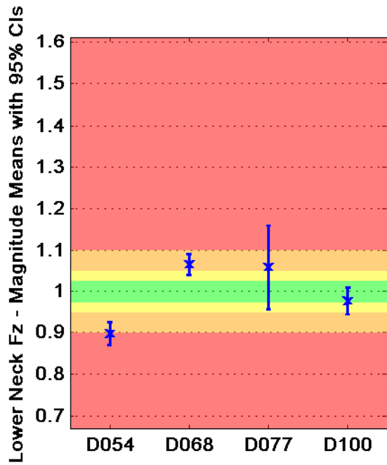
Taxicab Norm
