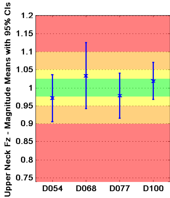
Taxicab Norm
