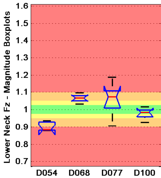
Taxicab Norm
