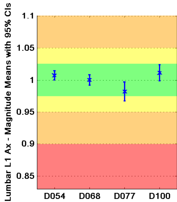
Taxicab Norm
