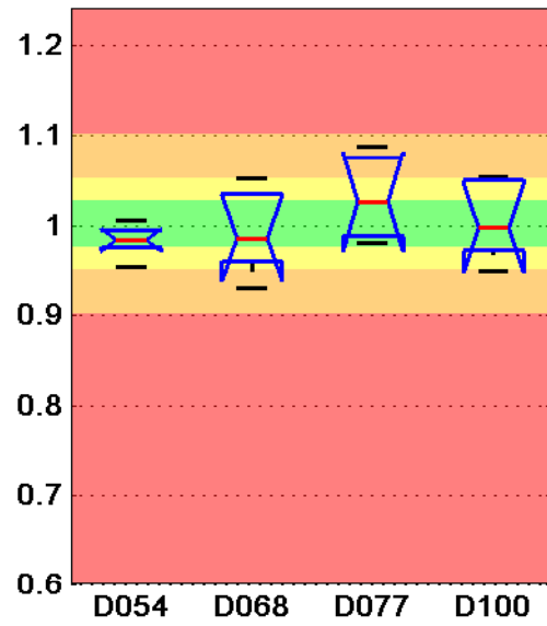
Euclidian Norm
