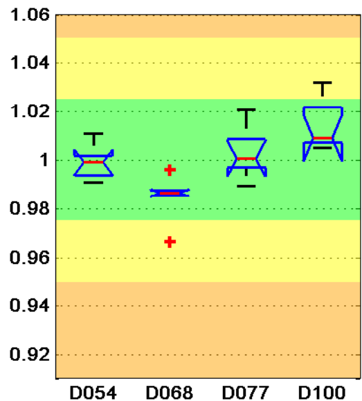
Euclidian Norm
