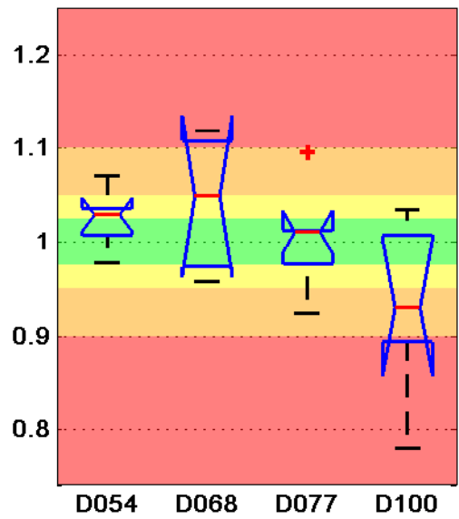
Euclidian Norm
