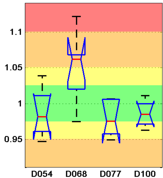
Euclidian Norm
