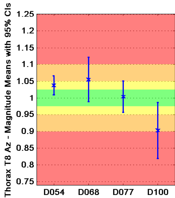
Taxicab Norm
