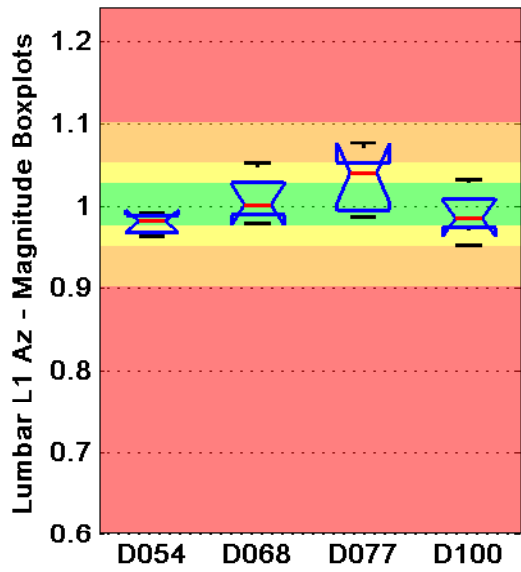
Taxicab Norm
