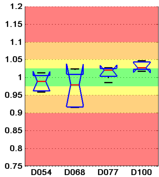
Euclidian Norm
