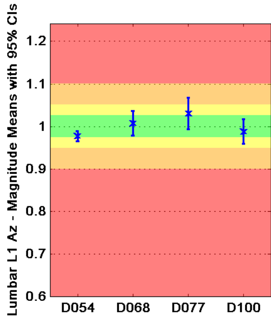
Taxicab Norm
