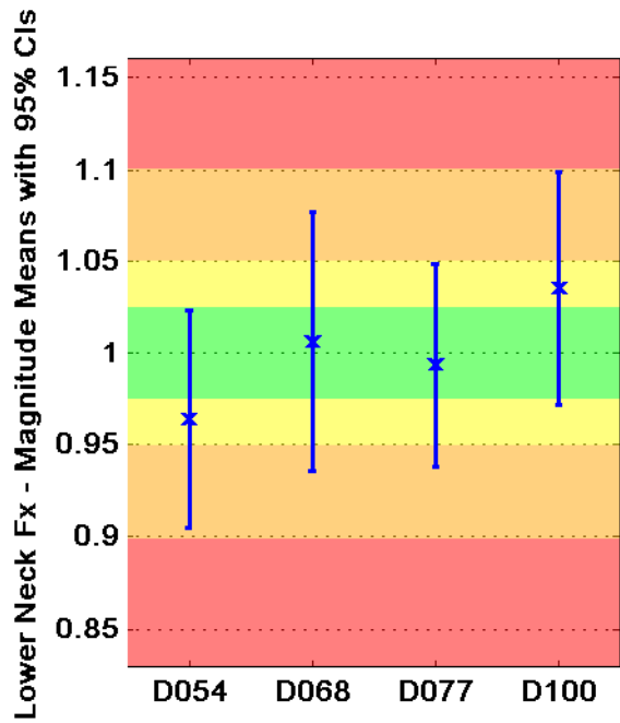
Taxicab Norm
