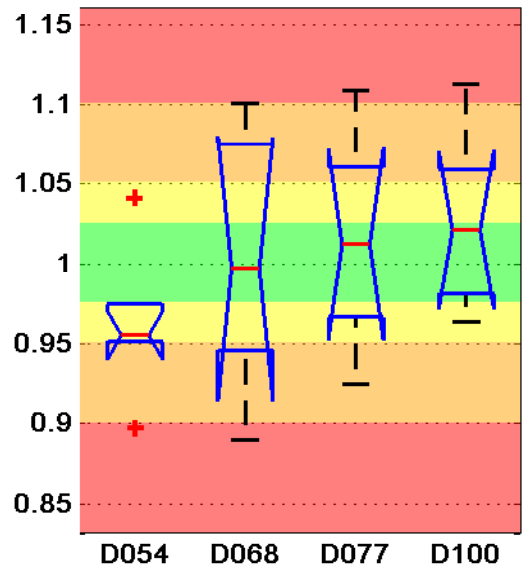
Euclidian Norm
