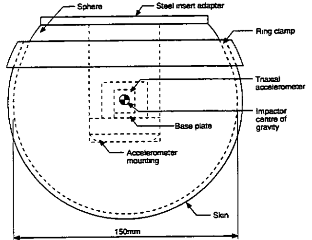
Figure 9. Adult headform impactor.
