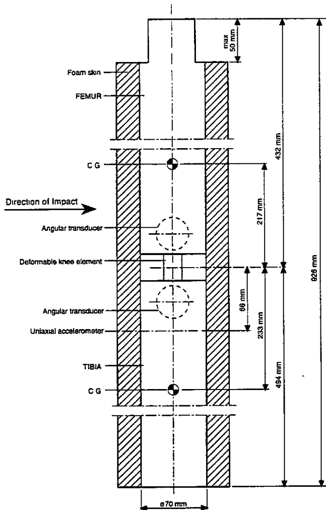
Figure 3. Legform impactor.
