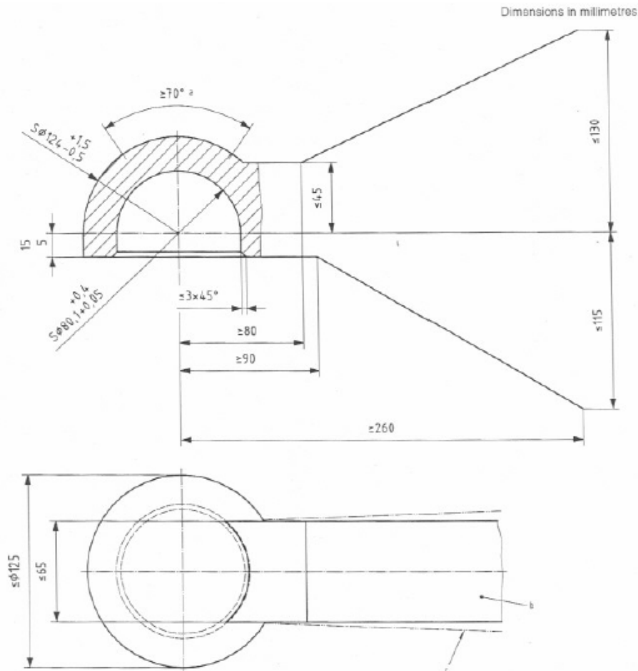
Figure 4 Dimensions of coupling head 80 of Class b
