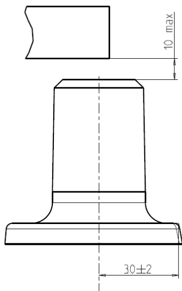
Figure 16 Position of the keeper plate
