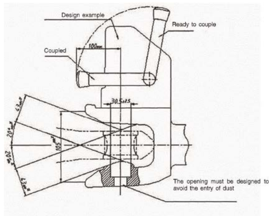
Figure 5 Automatic trailer coupling with cylindrical pin
