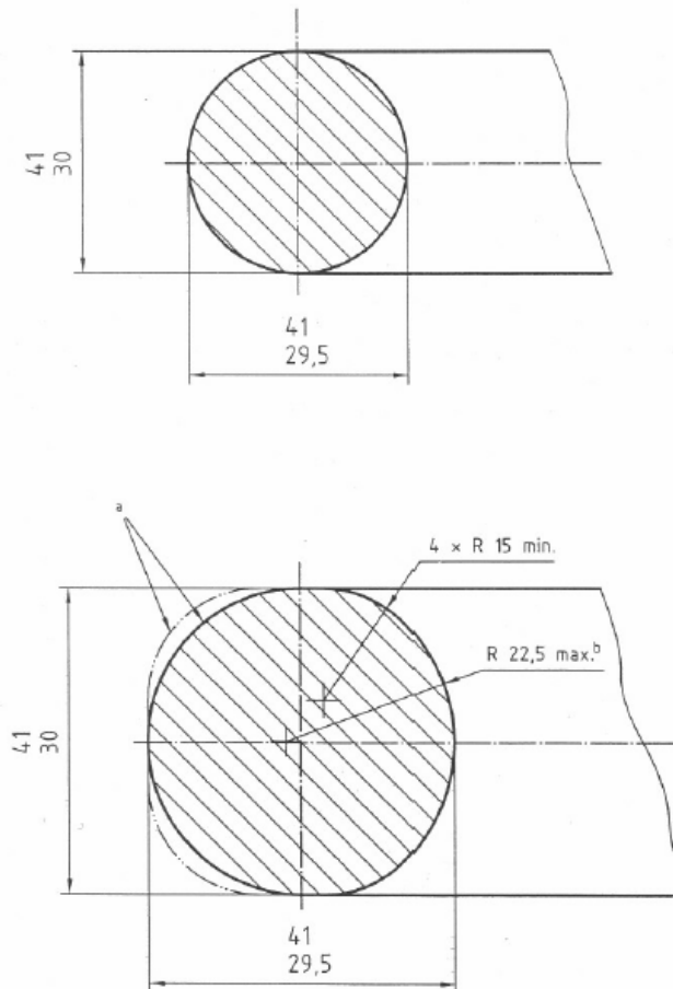
Figure 12 Dimensions of toroidal drawbar eye of class d50-2
