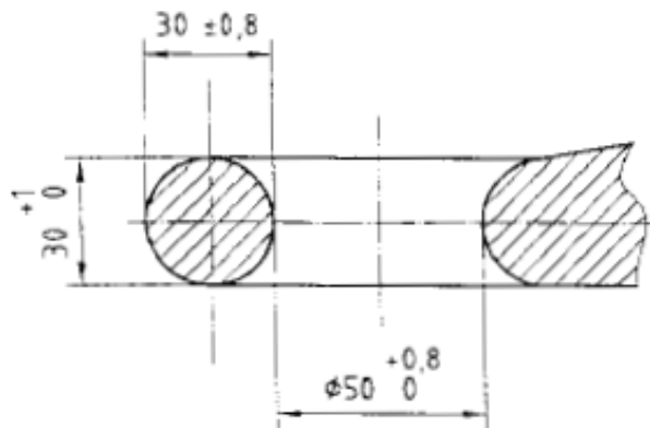
Figure 12 Dimensions of toroidal drawbar eye of class d50-2
