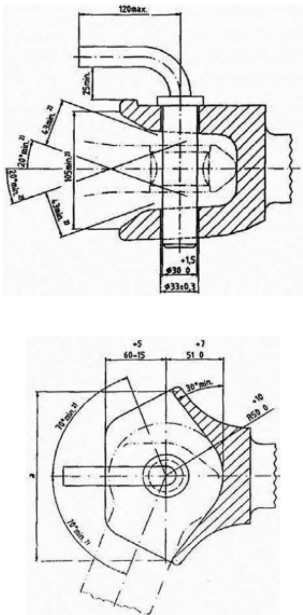
Figure 7 Non-automatic trailer coupling with cylindrical pin
