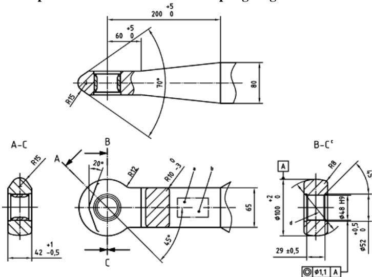
Figure 9 Principal dimensions of standard coupling ring d40-2
