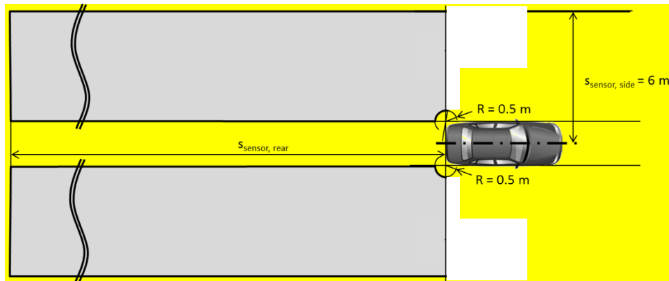
1 Figure Minimum detection area
