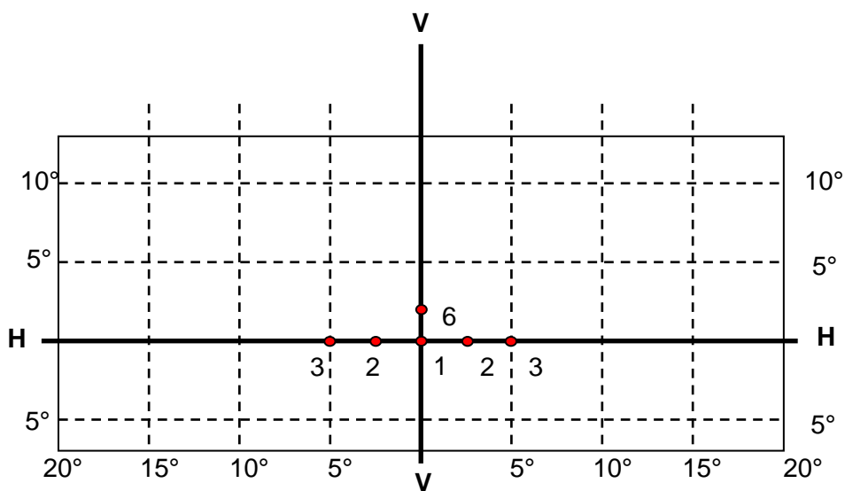
Figure D Secondary driving beam - position of test points
