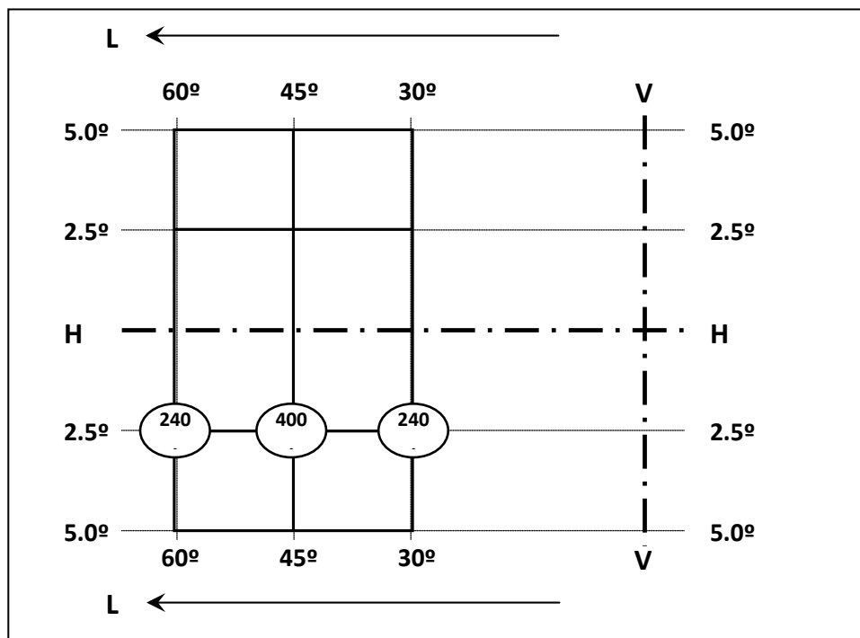
Figure L Measuring points for cornering lamps
