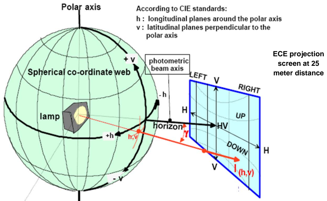
Spherical coordinate measuring system
