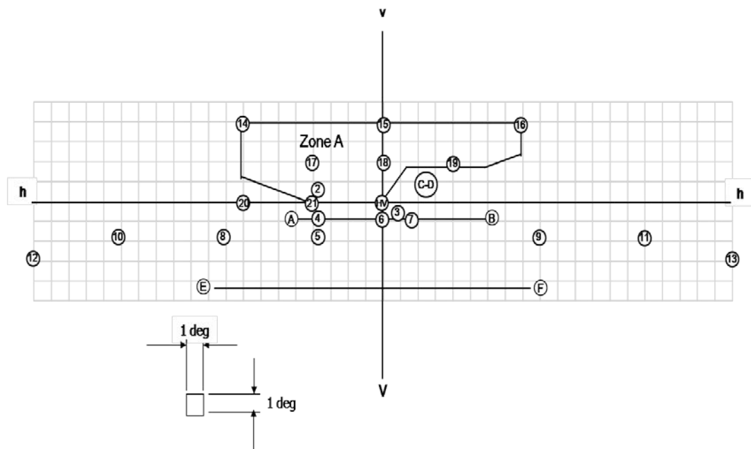
Figure F Passing beam with gas discharge light sources (GDL) for right-hand traffic
