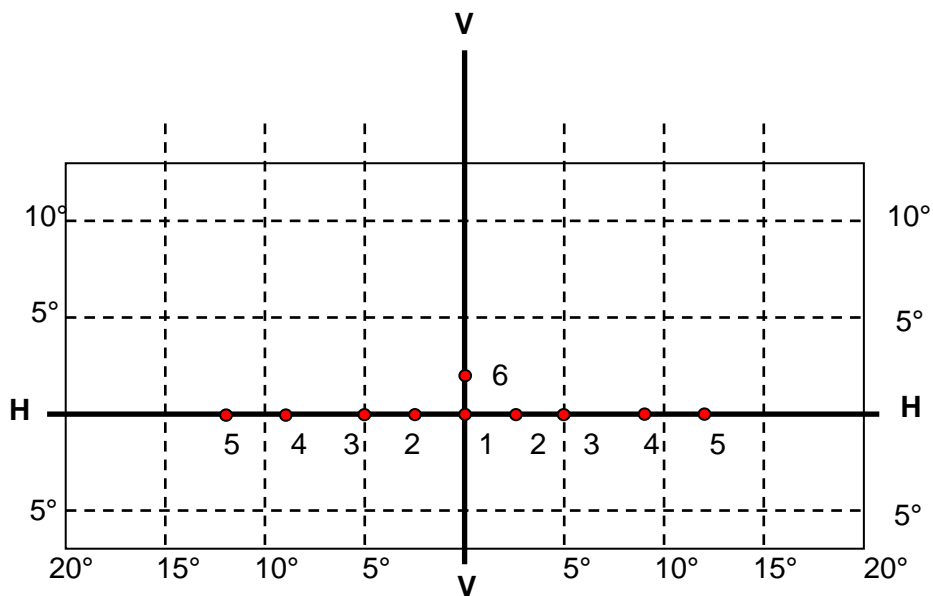
Figure C Primary driving beam - position of test points
