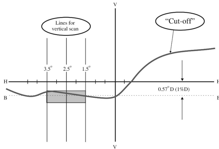
Figure A5-II Measurement of "cut-off" quality
