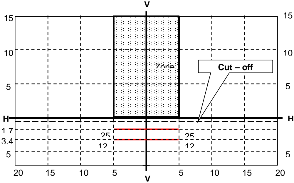
Figure H Passing beam test points and zones for Class AS headlamp(s):
