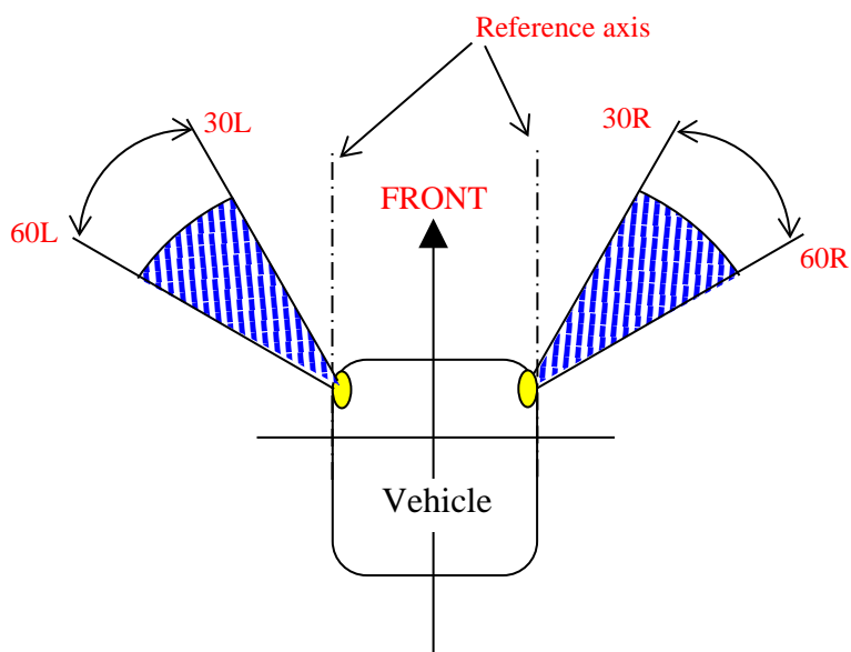
Figure M Horizontal geometric visibility for cornering lamps
