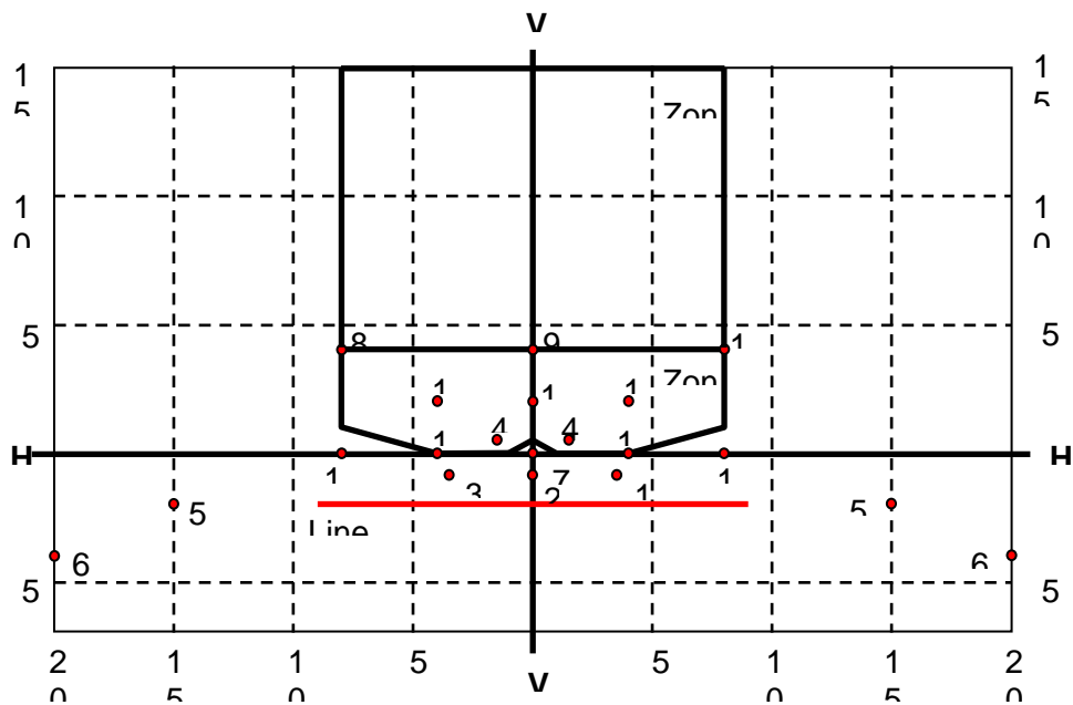
Figure J Passing beam - position of test points and zones for Classes CS, DS and ES headlamp(s):
