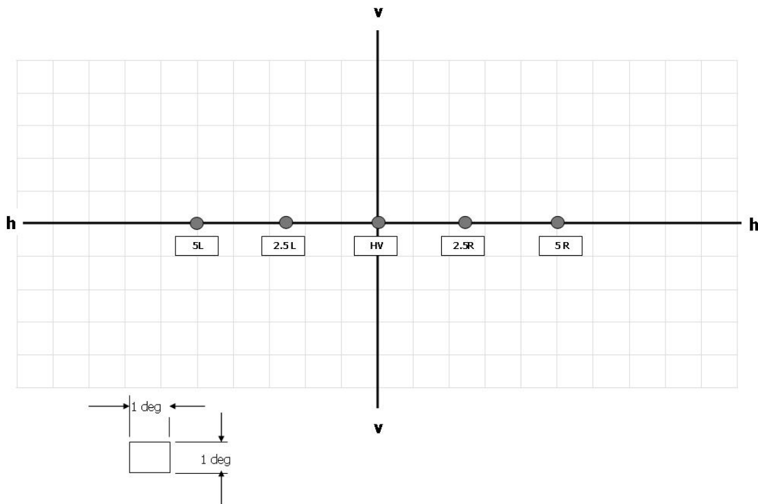
Figure B Driving beam test points
