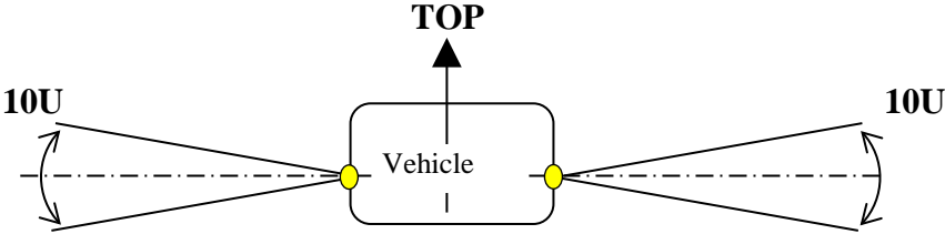
Figure N Vertical geometric visibility for cornering lamps
