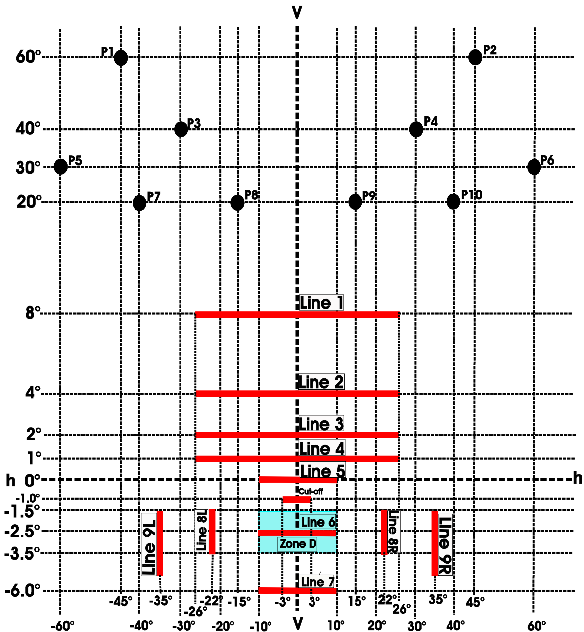
Figure K Light distribution of the Class F3 front fog lamp
