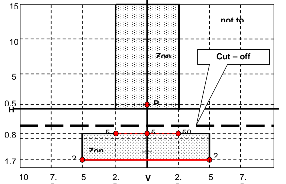
Figure I Passing beam test points and zones for Class BS headlamp(s):
