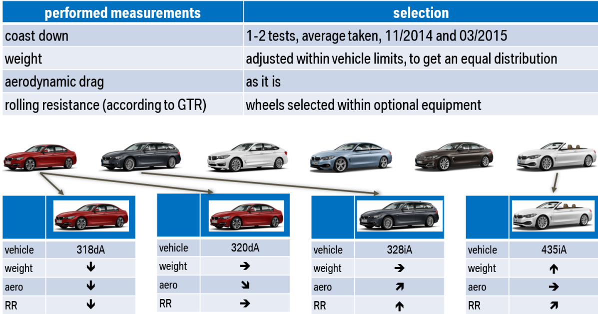
Figure 19 Results of the road load family validation tests
