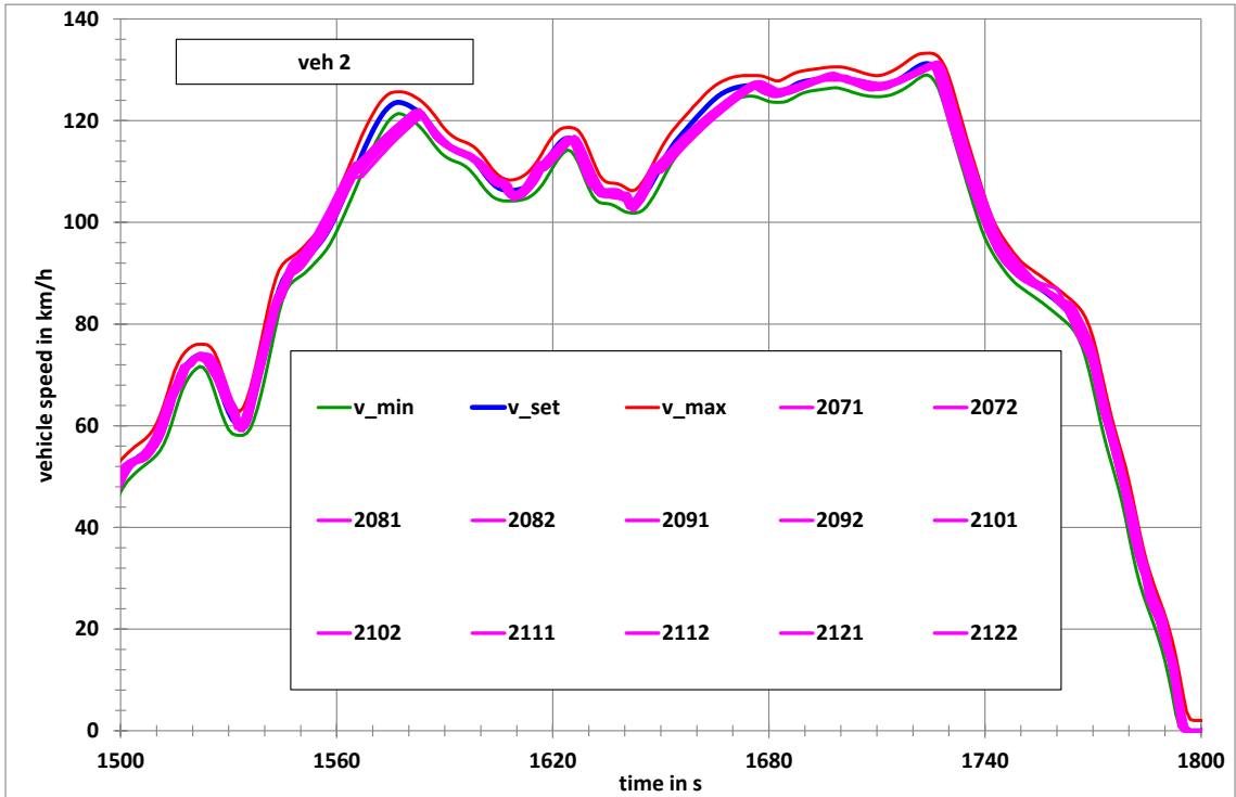
Figure 40 Example for tolerance band violations for the extra high speed phase of the class 3 WLTC (CNG fueled vehicle, power to mass ratio = 33.4 kW/t)
