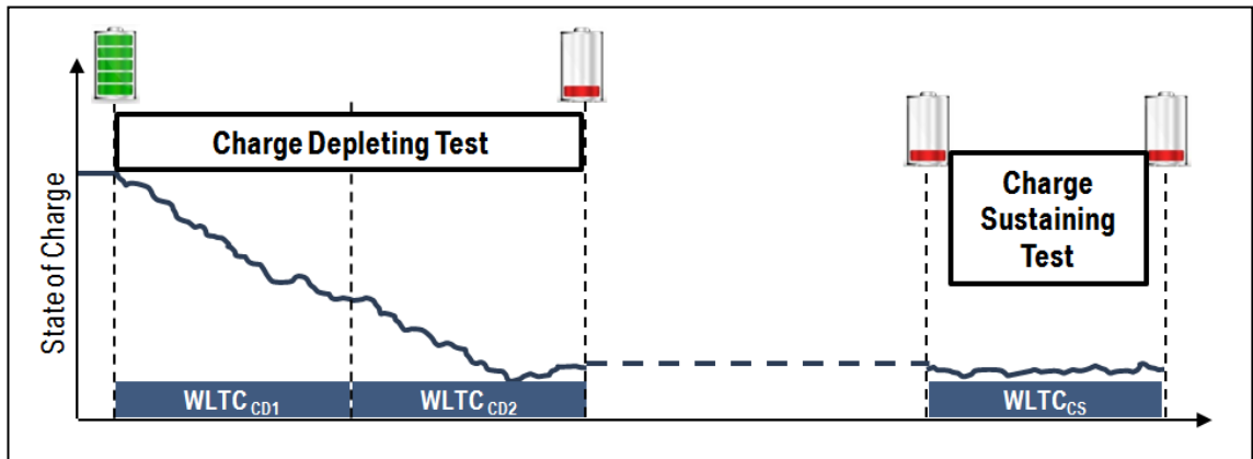
Figure 1 Procedure with charge depleting and sustaining test
