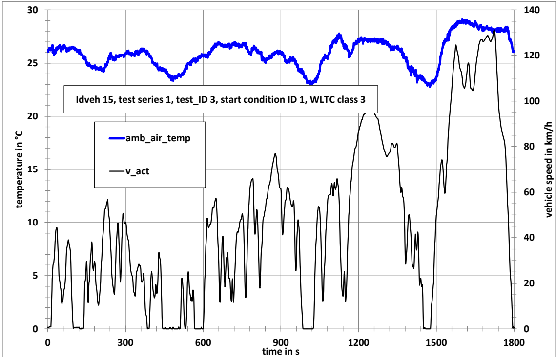
Figure 34 Worst case of test cell temperature over all four phases of the class 3 WLTC
