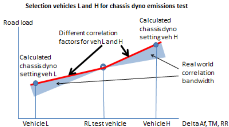
Figure 11 Example of the CO 2 interpolation method applied for road load relevant vehicle characteristics
