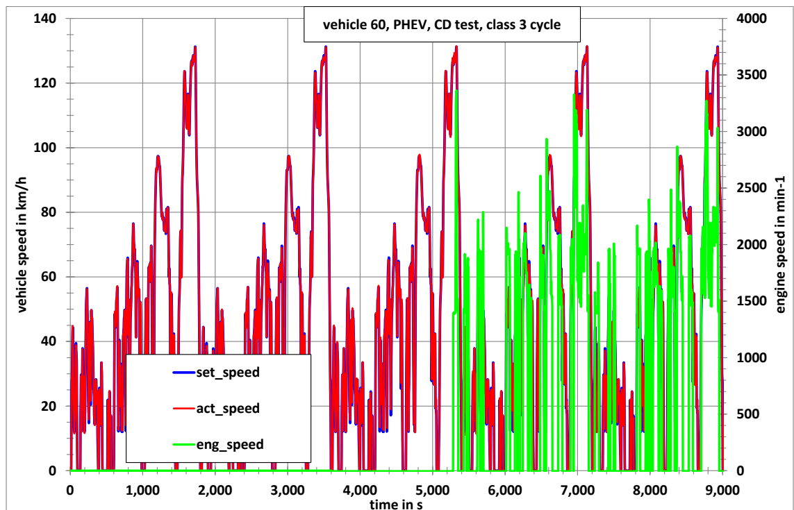
Charge depleting test for OVC-HEV vehicle 60, vehicle speed and engine speed
