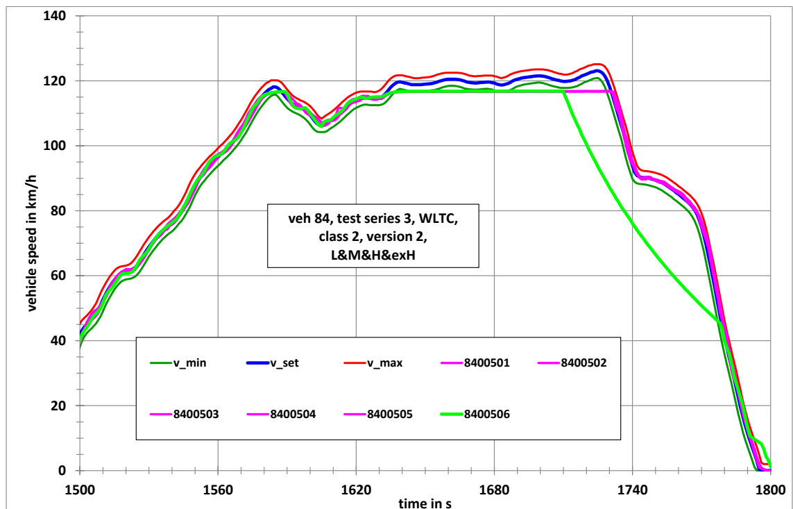
Time series of the vehicle speed for CD test 3 for vehicle 84 at break off section
