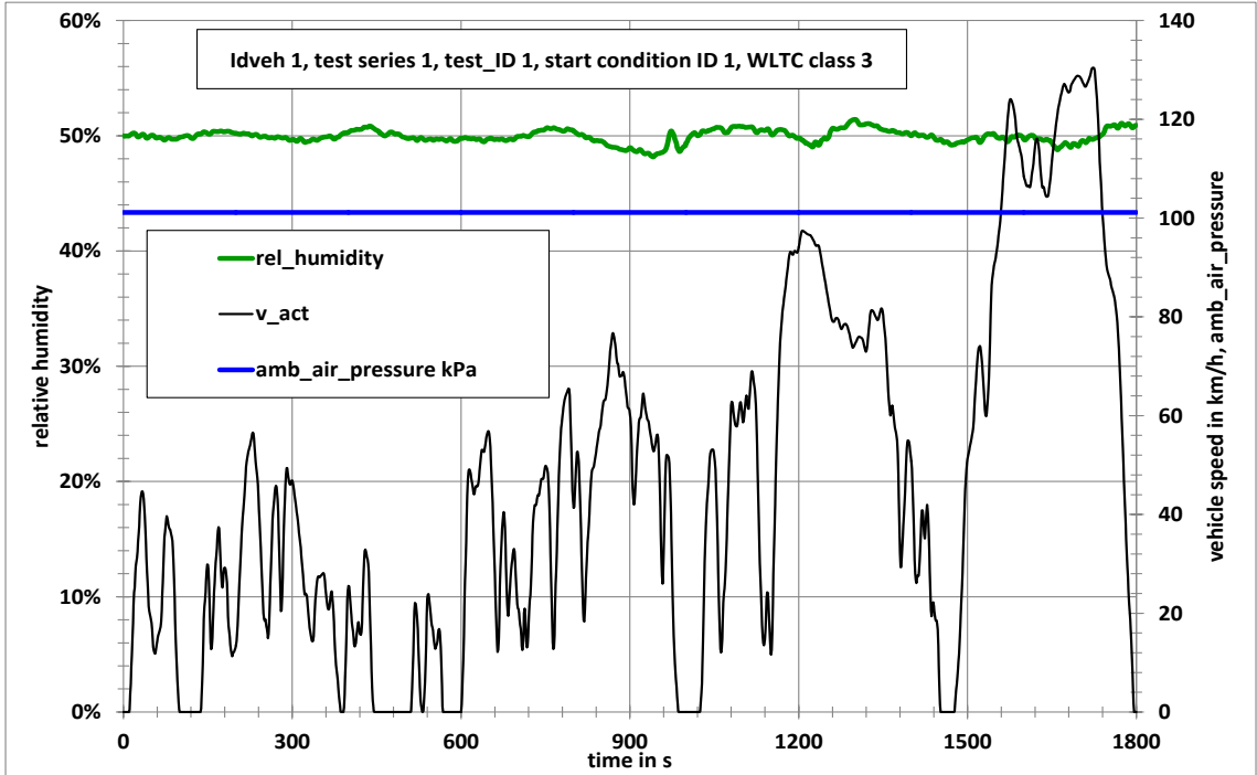
Figure 37 Example for the time history of the test cell humidity over the class 3 WLTC
