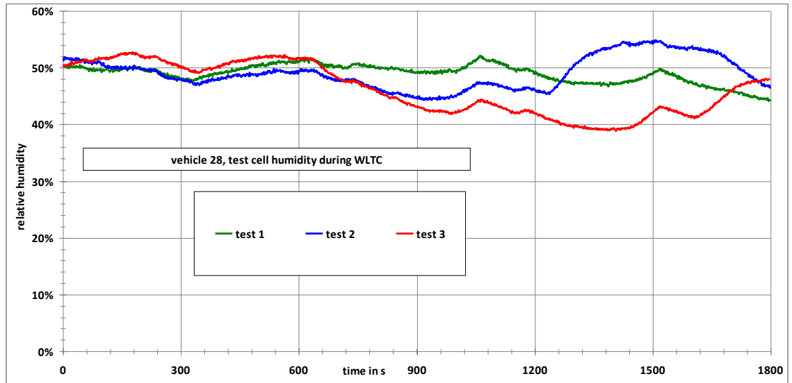
Figure 37 Example for the time history of the test cell humidity over the class 3 WLTC
