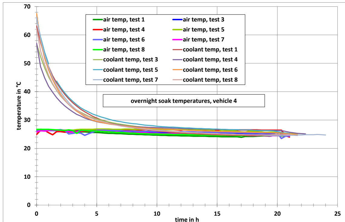
Example of overnight soak temperature monitoring
