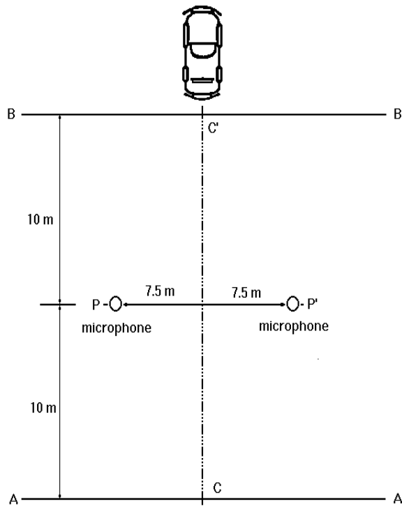
Figure 5 Microphone positions for the measurement
