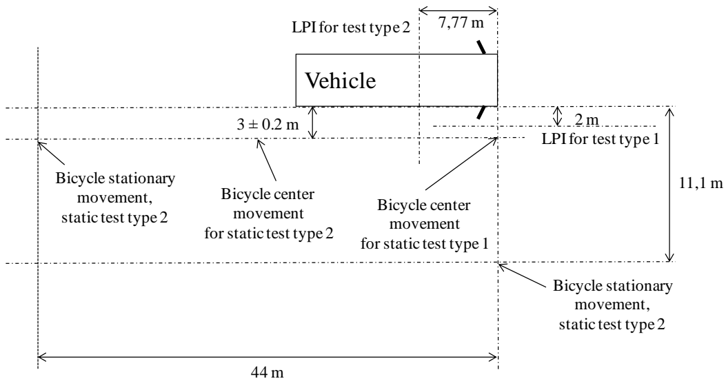
Figure 2: Static Tests
