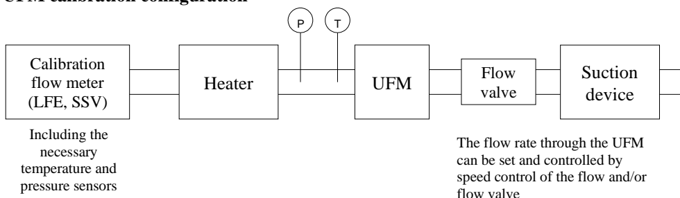
Figure A5/8 UFM calibration configuration
