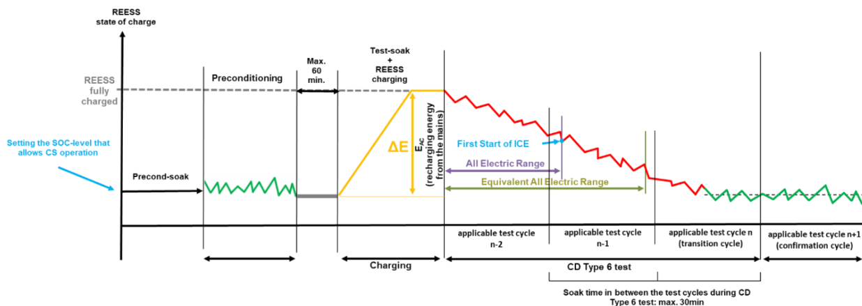
Figure A13.SA1.App1/1 OVC-HEVs, charge-depleting Type 6 test
