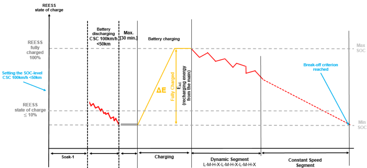
Figure A13.SA1.App1/8 PEV Type 6 test sequence
