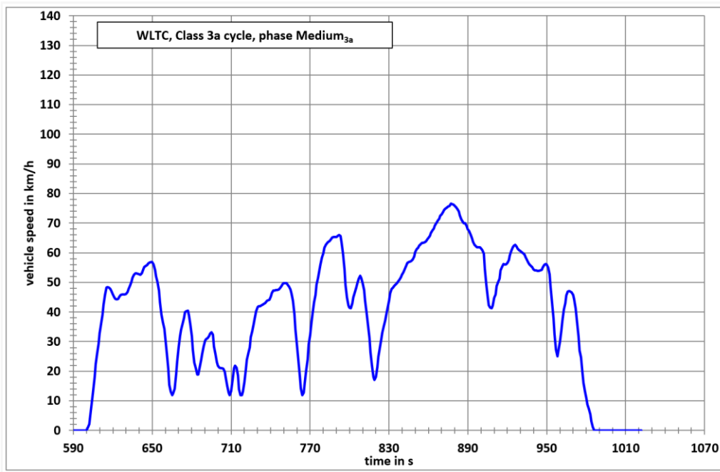
WLTC, Class 3a cycle, phase Medium 3a
