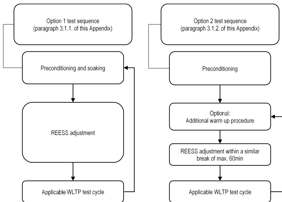
Figure A8.App2/1 OVC-HEV and OVC-FCHV test sequences
