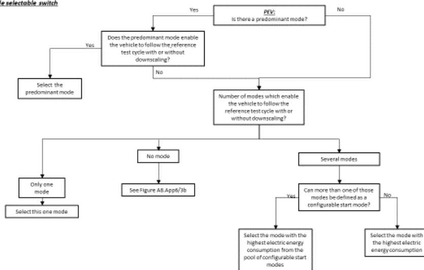
Figure A8.App6/3a PEV: Mode selectable switch
