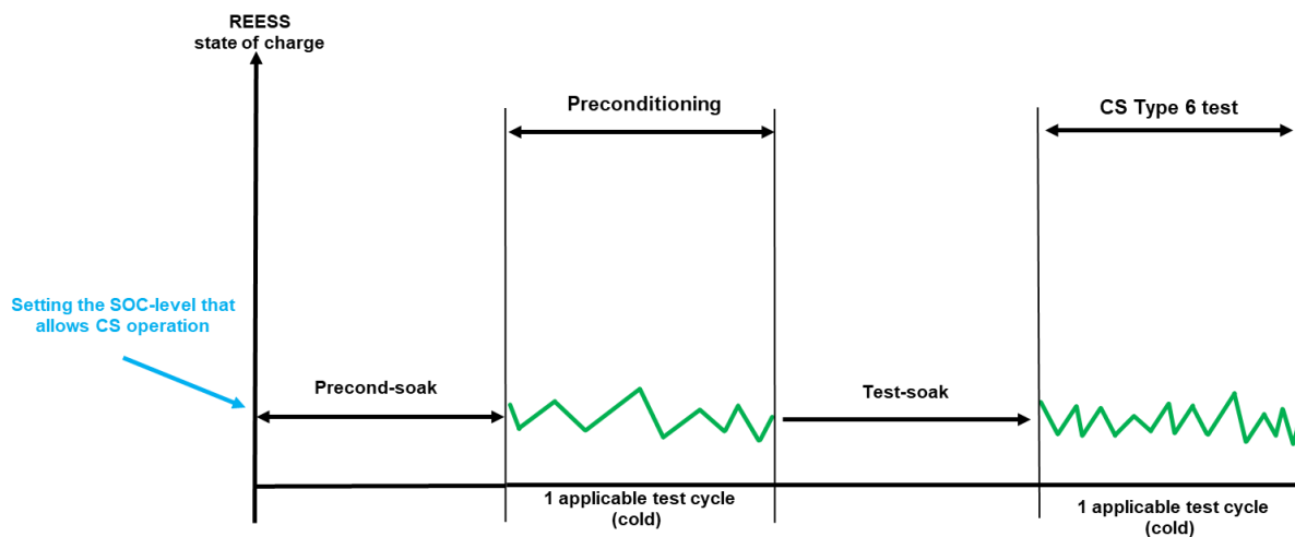
Figure A13.SA1.App1/7 NOVC-HEVs charge-sustaining Type 6 test
