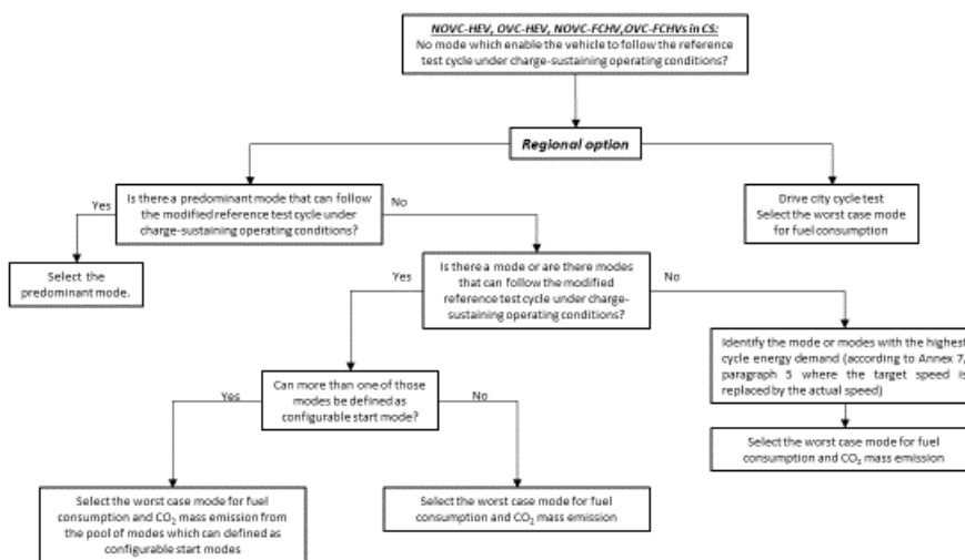
Figure A8.App6/2b NOVC-HEV, OVC-HEVs, NOVC-FCHV, OVC-FCHVs in CS: CS Type 1 Test – Mode selectable switch
