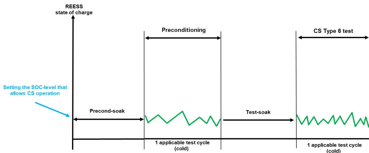
Figure A13.SA1.App1/2 OVC-HEVs, charge-sustaining Type 6 test
