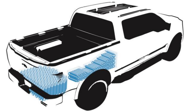
Type IV carbon fiber conformable H2 tank 70MPa
