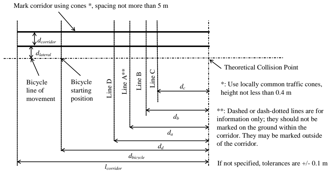
Figure 1 Dynamic tests
