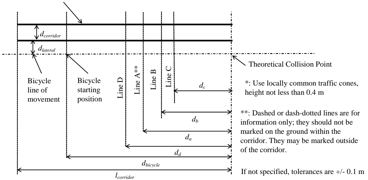
Figure 2 Static tests
