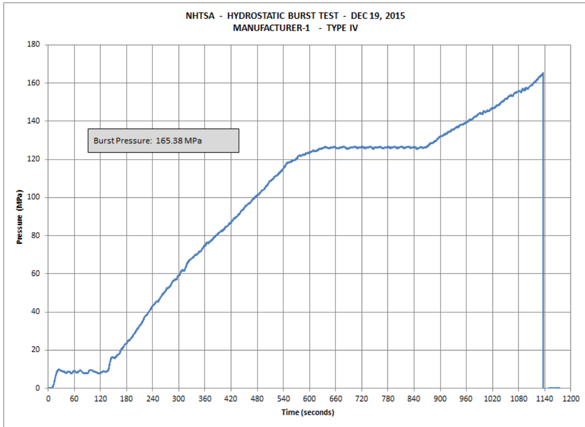
Figure 43. Hydraulic Sequence Burst Test - Pressure Plot of Container 1-E
