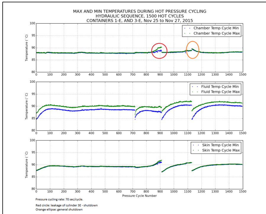
Figure 40. Temperatures recorded during hot pressure cycling
