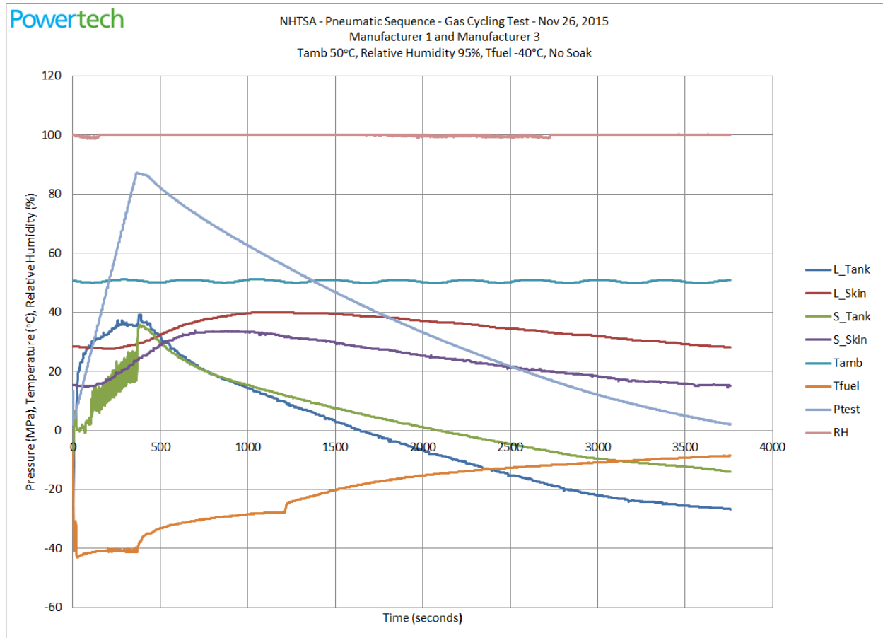
Figure 52. Gas Cycling Test Stage 5 – hot cycles, full cycle
