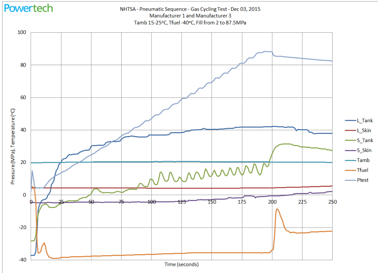
Figure 55. Gas Cycling Test Stage 6 – ambient cycles, fill profile
