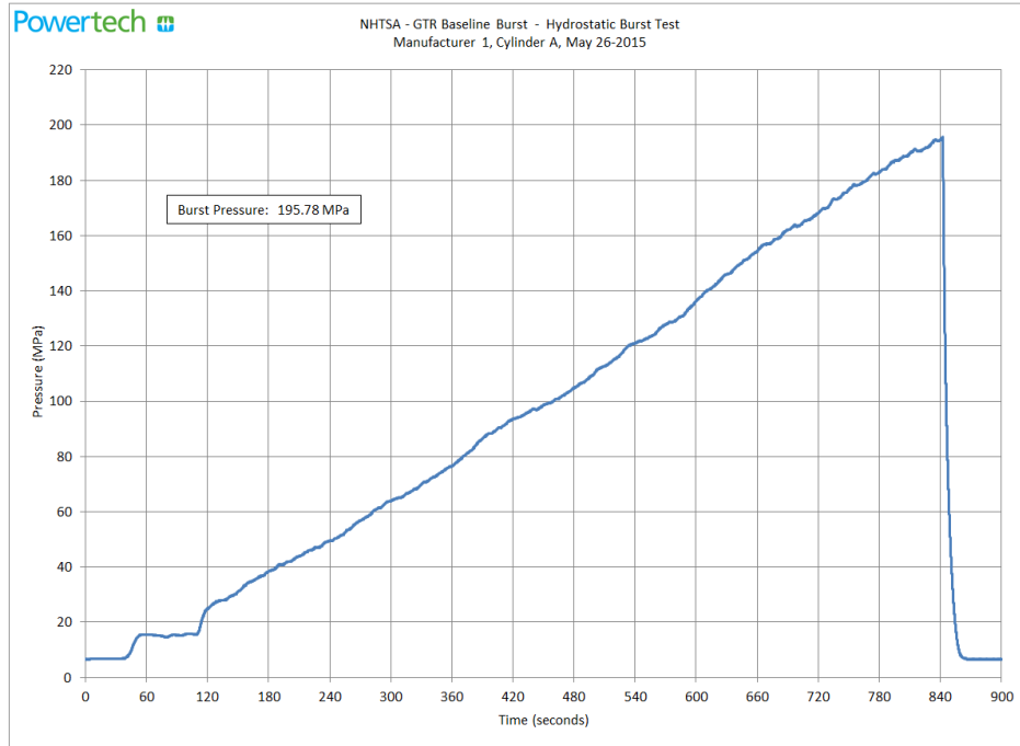
Figure 26. Baseline Burst Pressure Plot of Container 1-A
