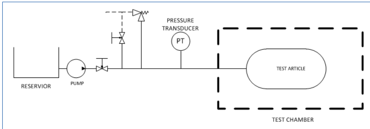
Figure 3. Proof Pressure Test Setup
