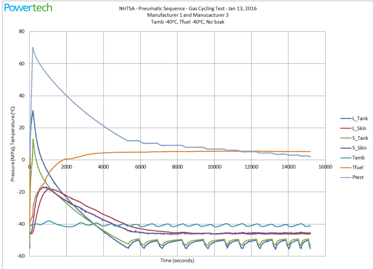
Figure 58. Gas Cycling Test Stage 9 – cold cycles, full cycle
