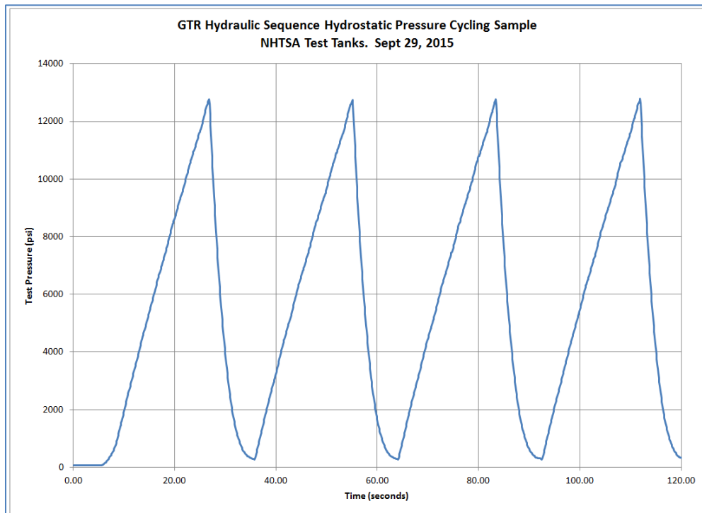
Figure 35. Hydraulic Sequence Ambient Pressure Cycling Profile
