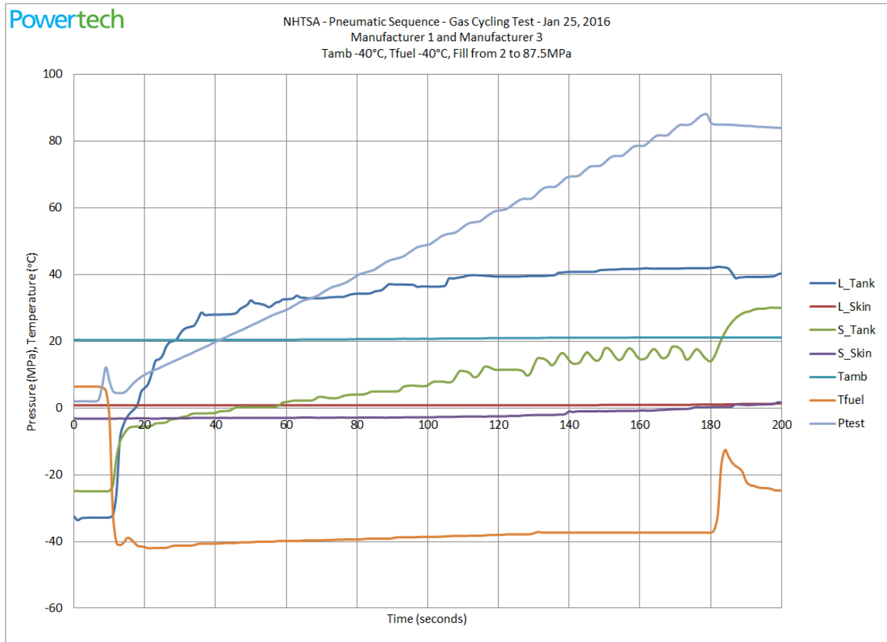
Figure 61. Gas Cycling Test Stage 10 – ambient cycles, fill profile
