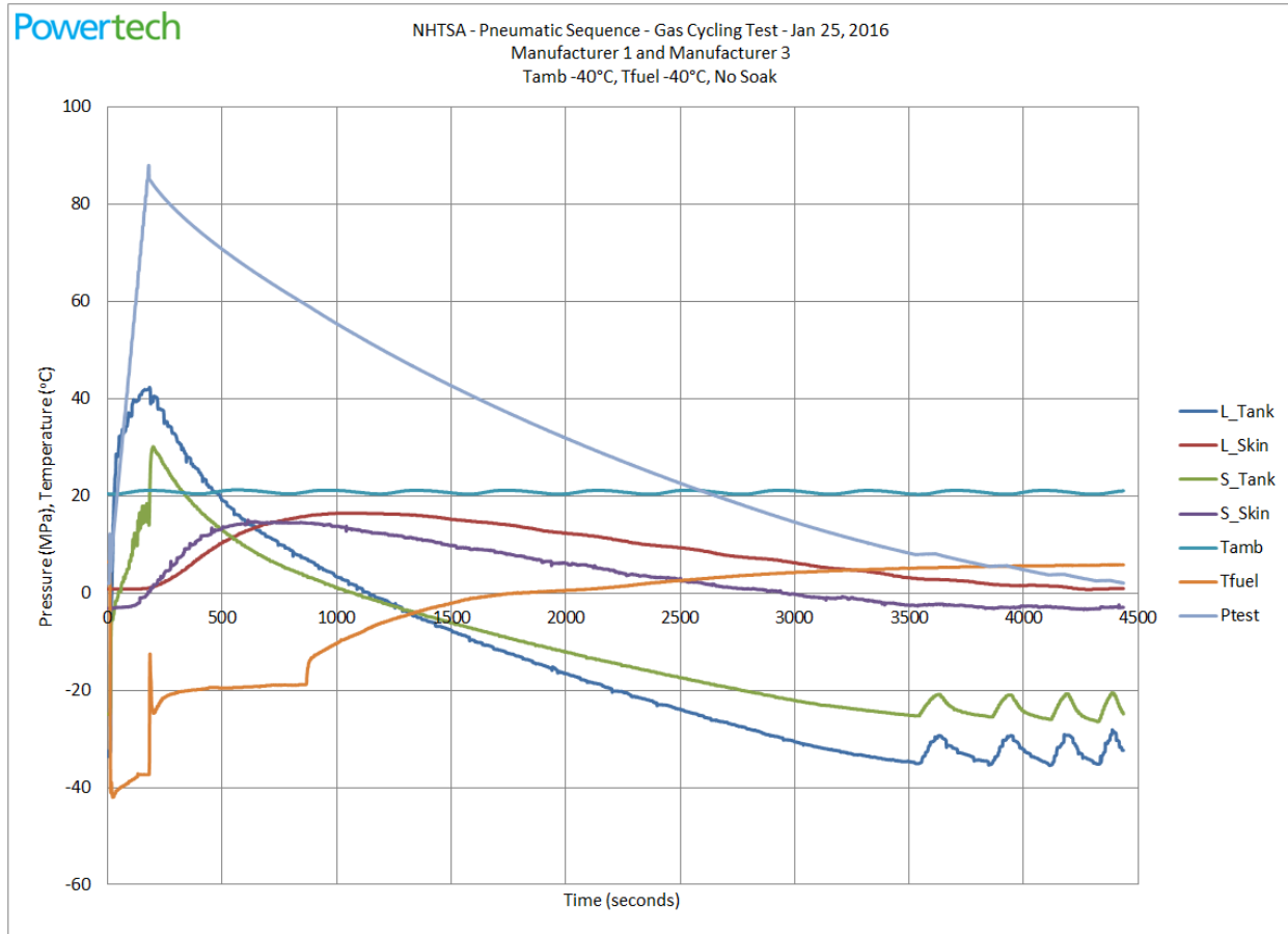
Figure 60. Gas Cycling Test Stage 10 – ambient cycles, full cycle
