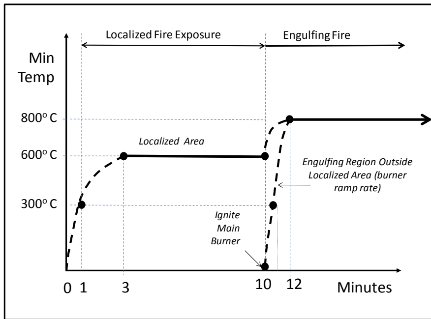
Figure 24. Localized Fire Test Temperature Profile
