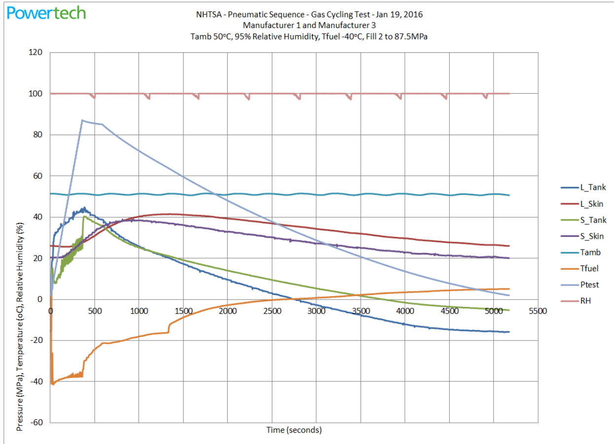
Figure 56. Gas Cycling Test Stage 8 – hot cycles, full cycle
