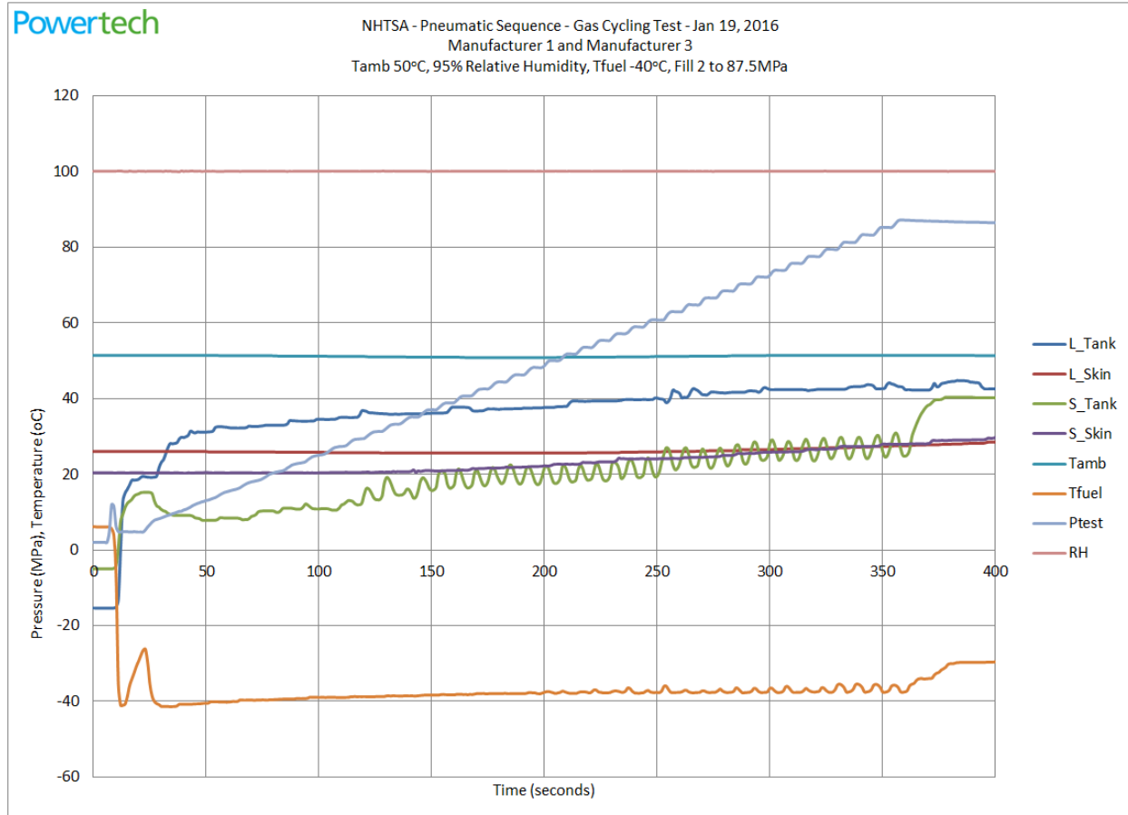
Figure 57. Gas Cycling Test Stage 8 – hot cycles, fill profile
