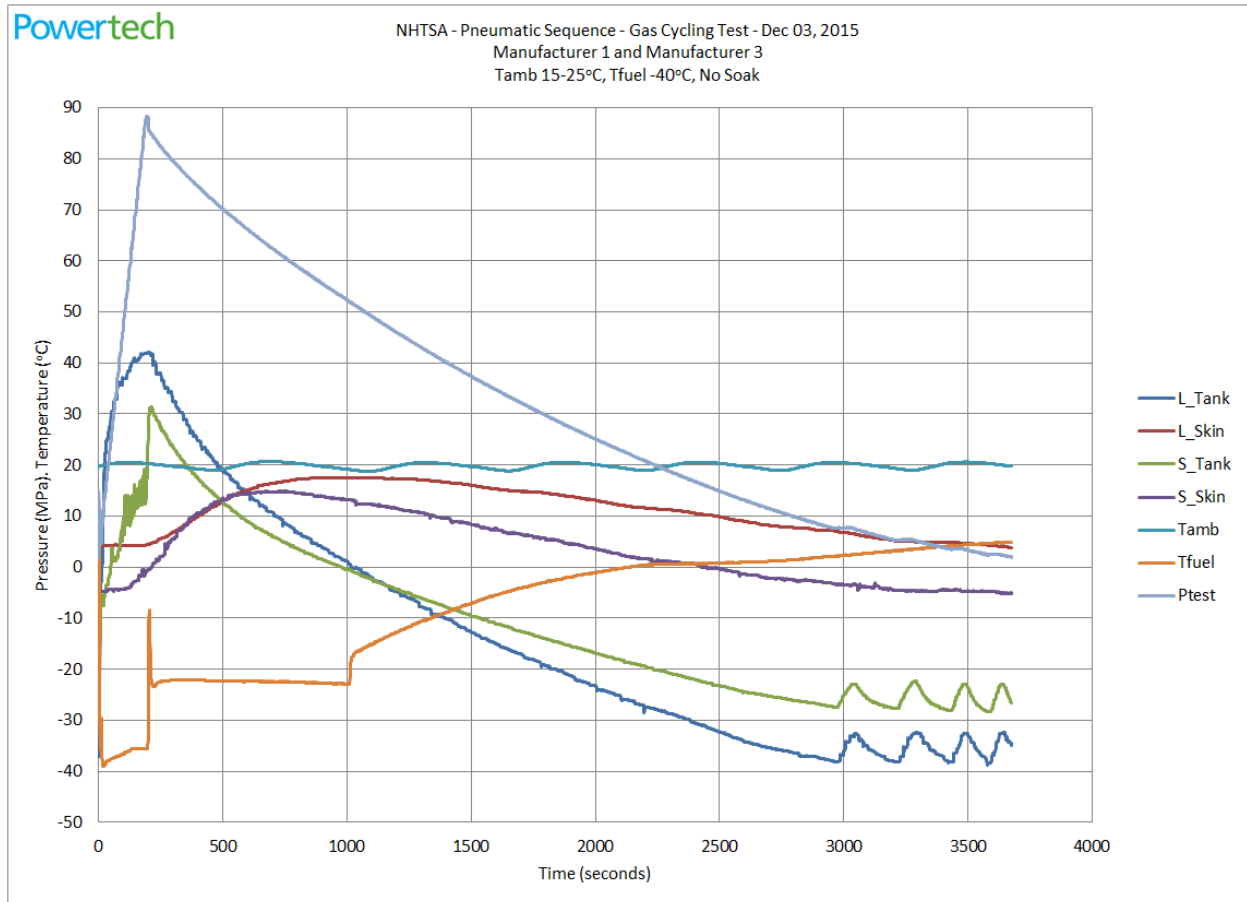
Figure 54. Gas Cycling Test Stage 6 – ambient cycles, full cycle
