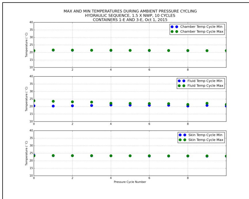
Figure 37. Max and Min Temperatures during last 10 ChemEx Ambient Cycles to 1.5 x NWP
