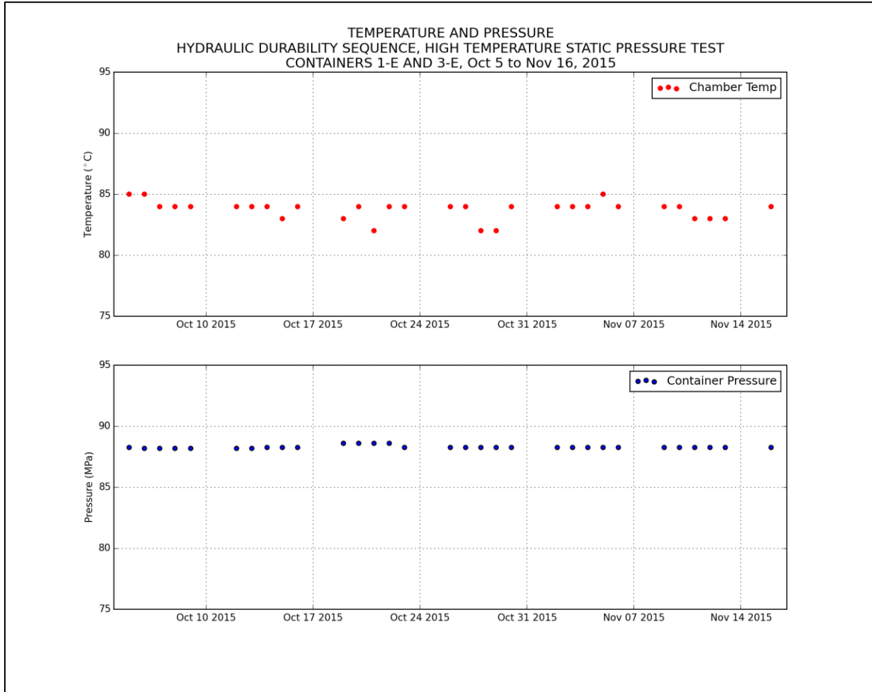
Figure 38. Temperatures and pressures during high temperature static pressure sequence
