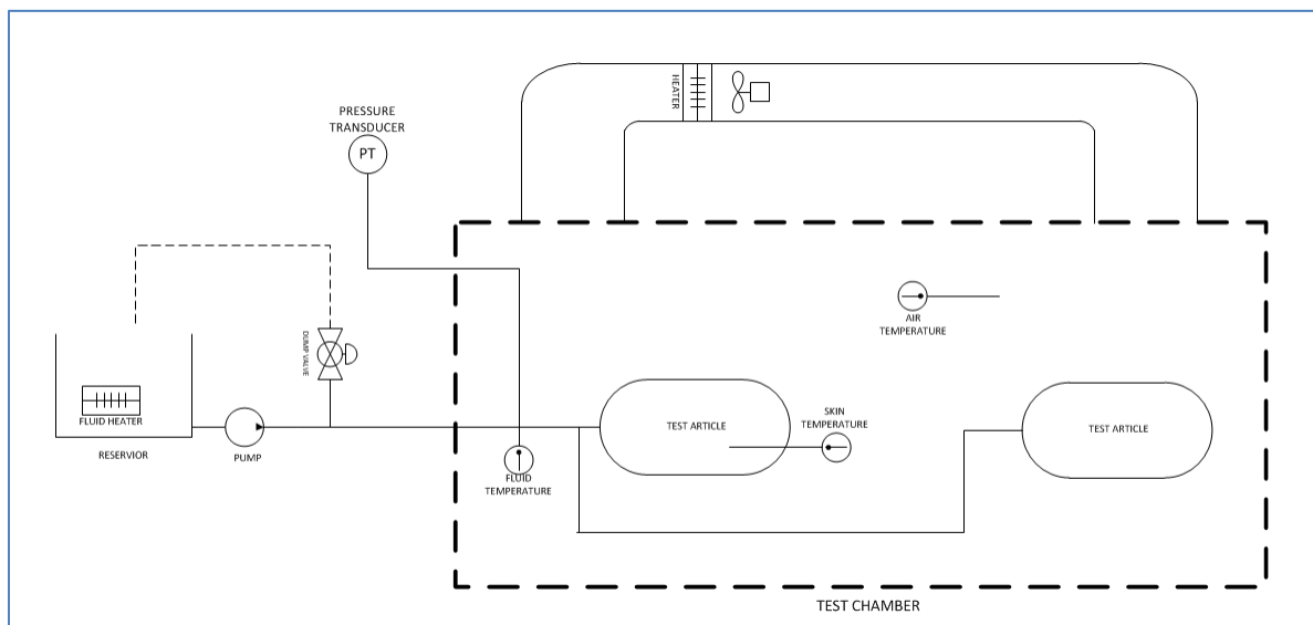
Figure 16. Hot Pressure Cycling Test Setup
