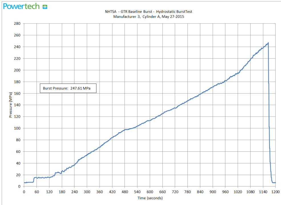
Figure 32. Baseline Burst Pressure Plot of Container 3-A
