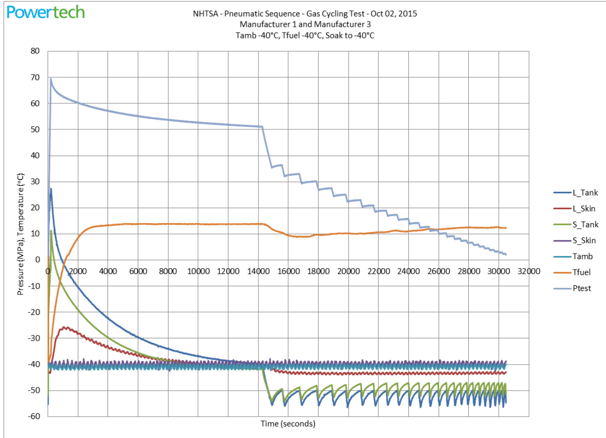
Figure 46. Gas Cycling Test Stage 2 – cold soak cycles with -40°C fuel delivery temperature, full cycle
