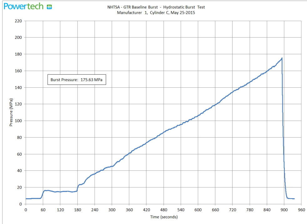
Figure 28. Baseline Burst Pressure Plot of Container 1-C
