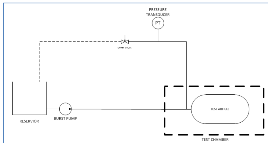
Figure 23. Residual Strength Burst Test Setup
