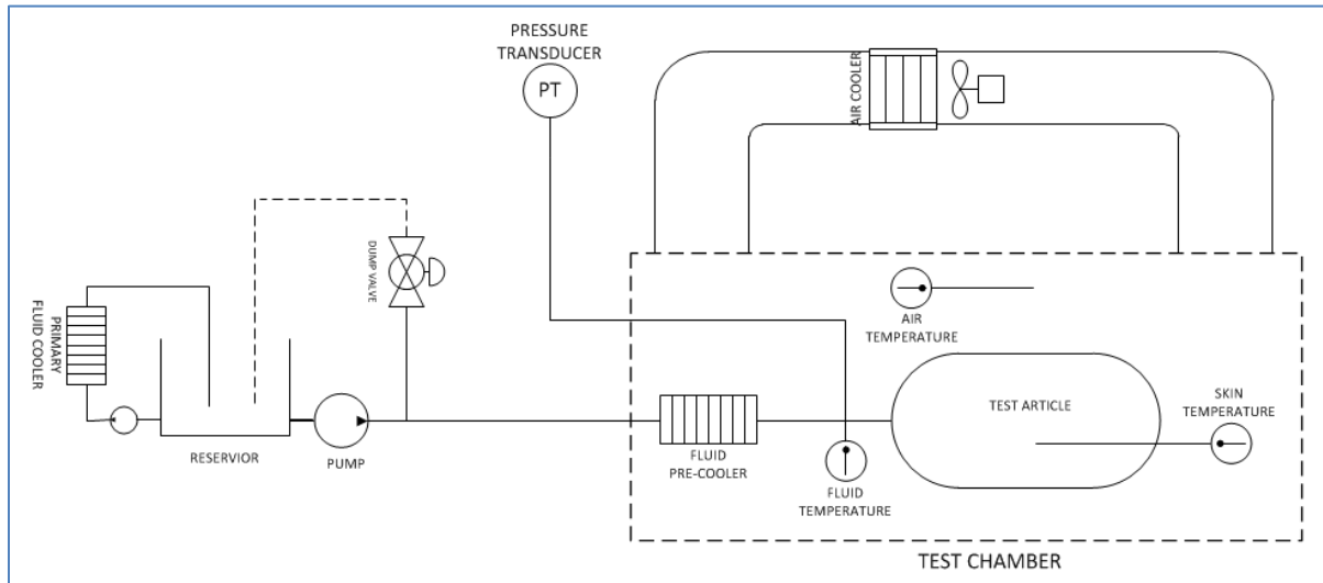
Figure 15. Cold Pressure Cycling Test Setup
