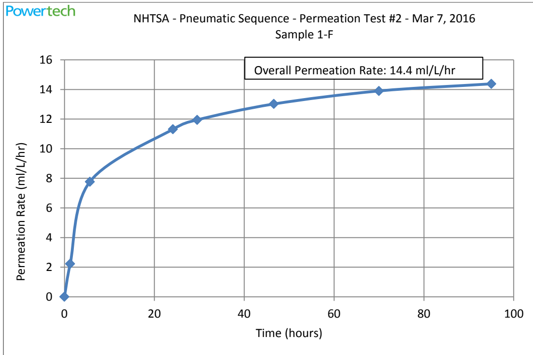
Figure 64. Permeation Test #2, Container 1-F
