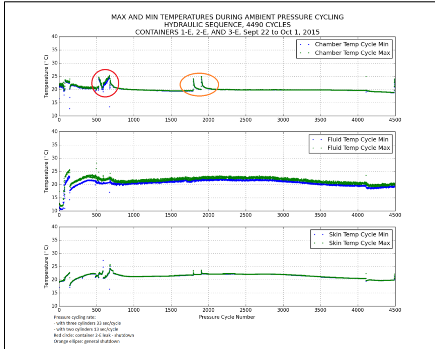
Figure 36. Max and Min Temperatures during ChemEx Ambient Cycles to 1.25xNWP
