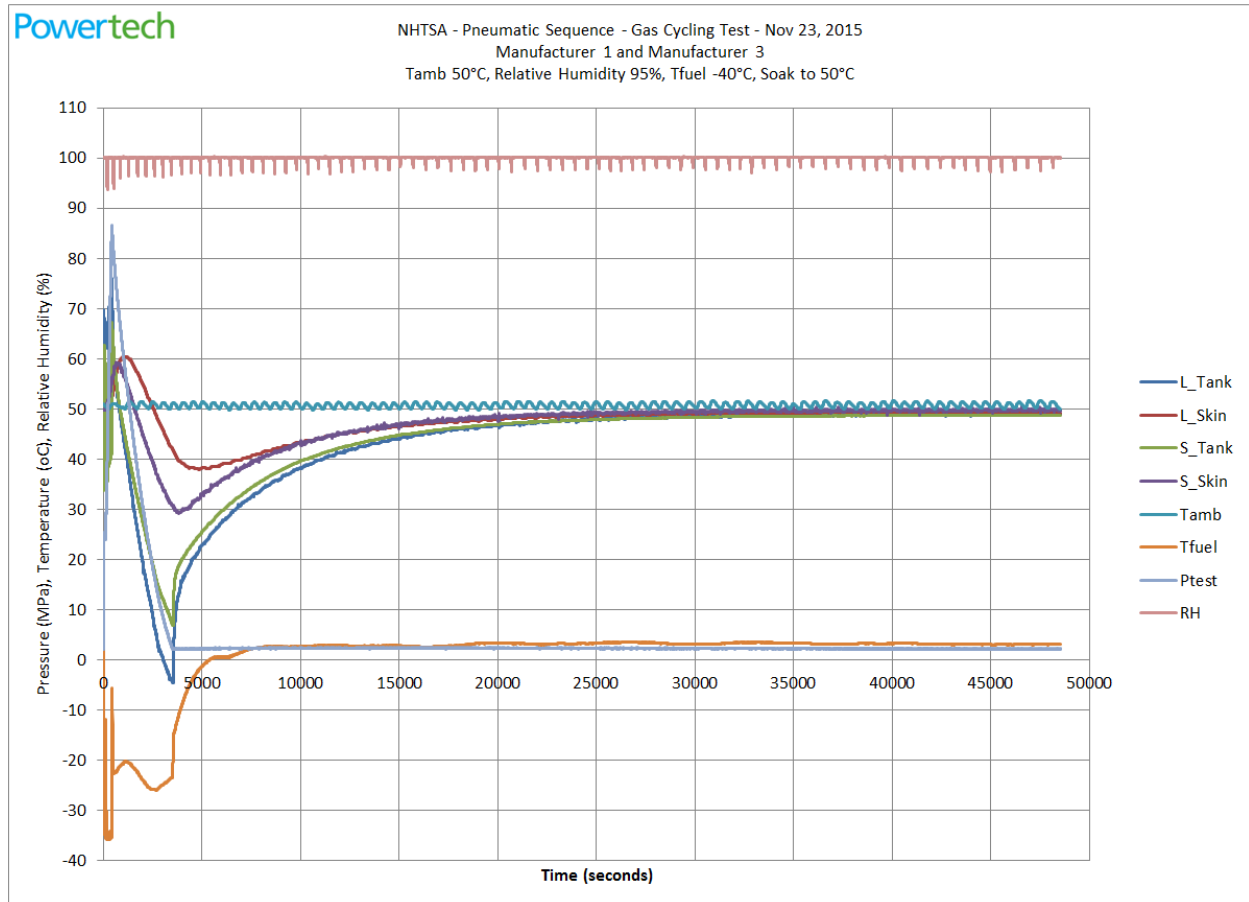
Figure 50. Gas Cycling Test Stage 4 – hot soak cycles, full cycle
