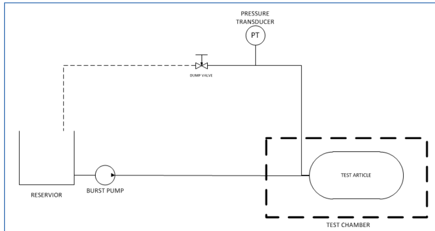
Figure 18. Hydraulic Residual Pressure Test and Burst Test Setup
