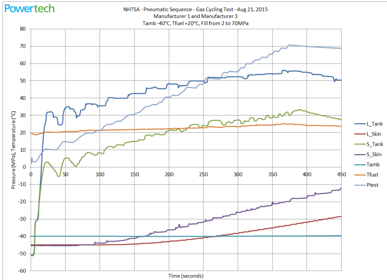
Figure 45. Gas Cycling Test Stage 1 – cold soak cycles with 20°C fuel delivery temperature, fill profile
