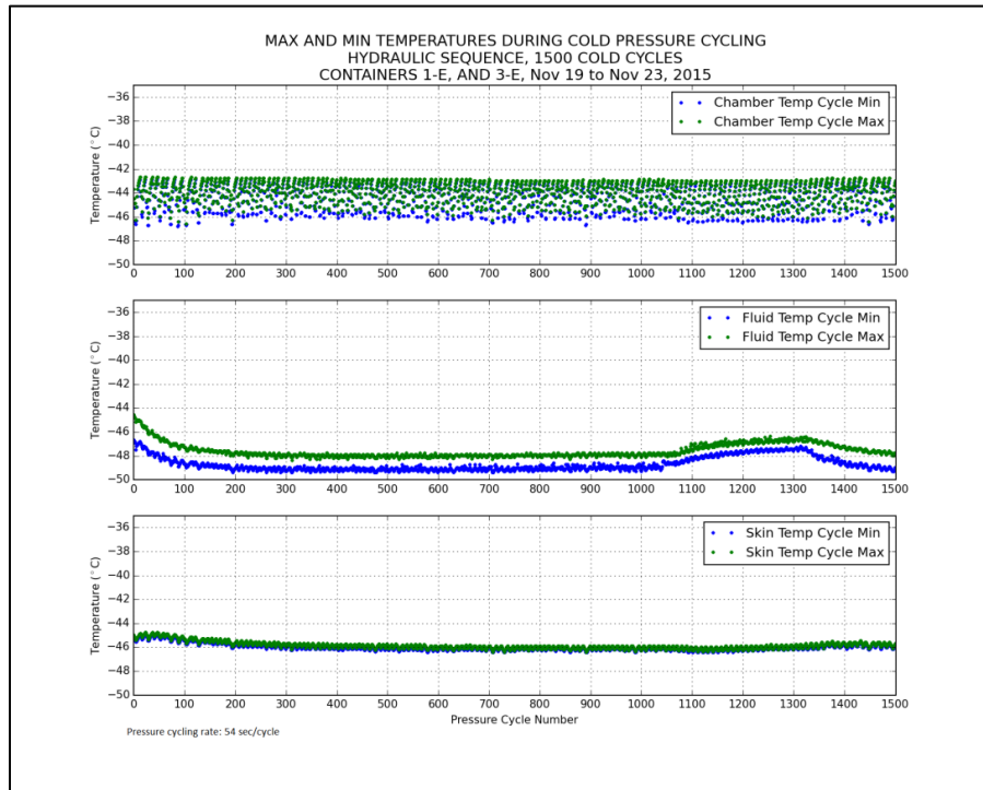
Figure 39. Temperatures recorded during cold pressure cycling
