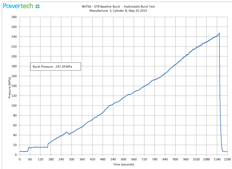
Figure 33. Baseline Burst Pressure Plot of Container 3-B
