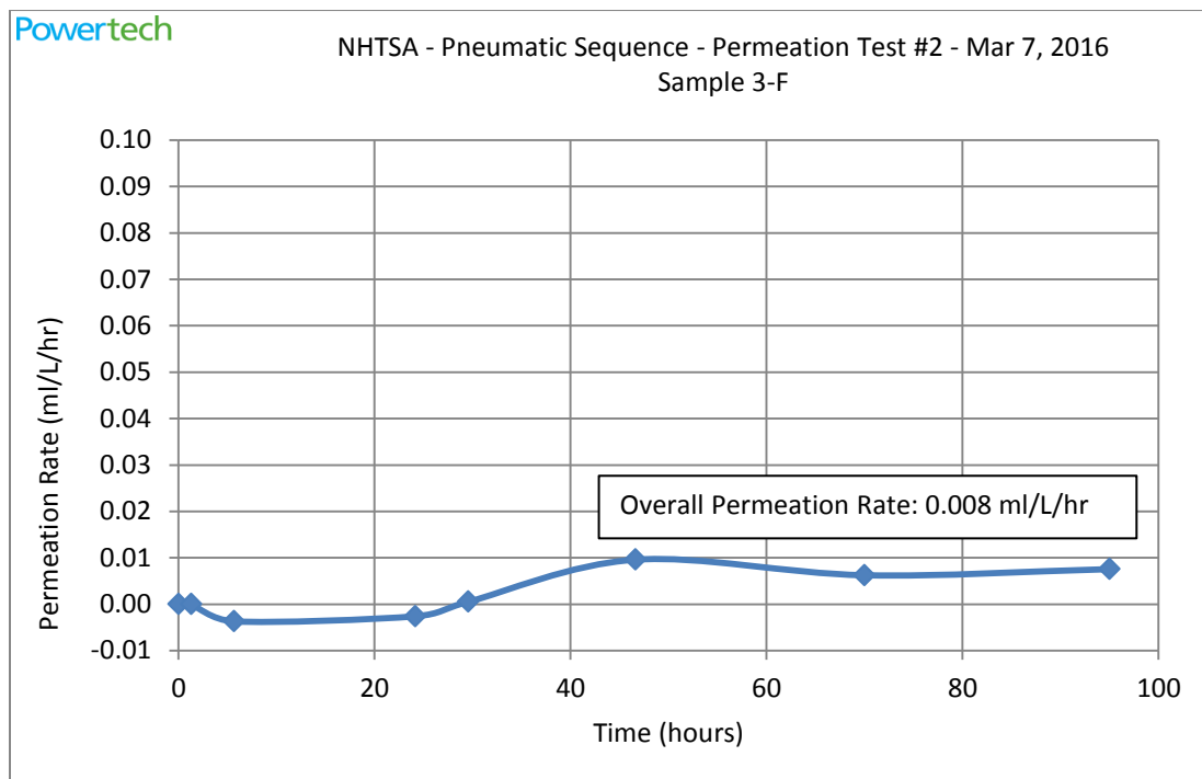
Figure 65. Permeation Test #2, Container 3-F
