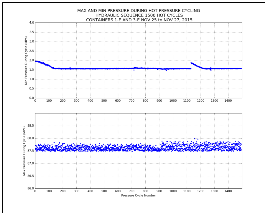
Figure 42. Max and min pressures recorded during hot pressure cycling
