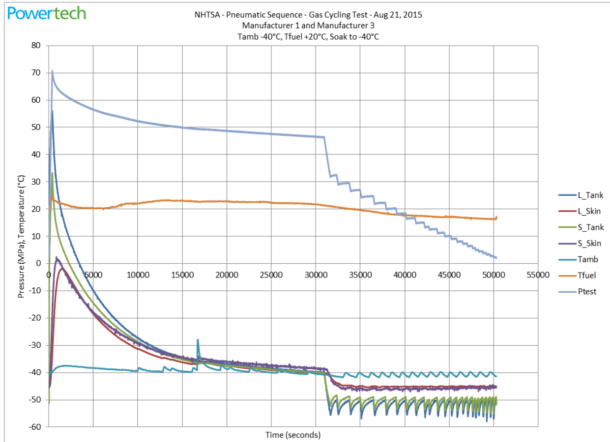
Figure 44. Gas Cycling Test Stage 1 – cold soak cycles with 20°C fuel delivery temperature, full cycle
