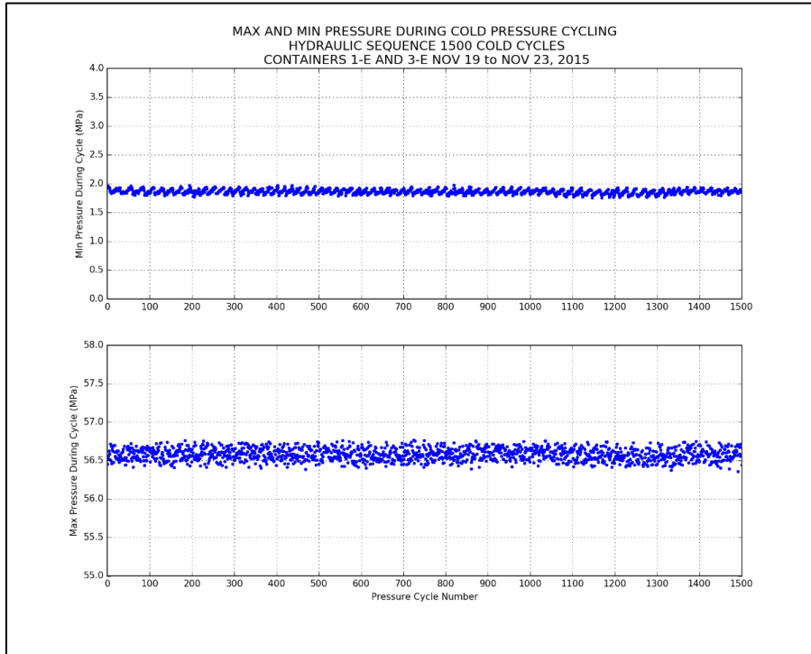
Figure 41. Max and min pressures recorded during cold pressure cycling
