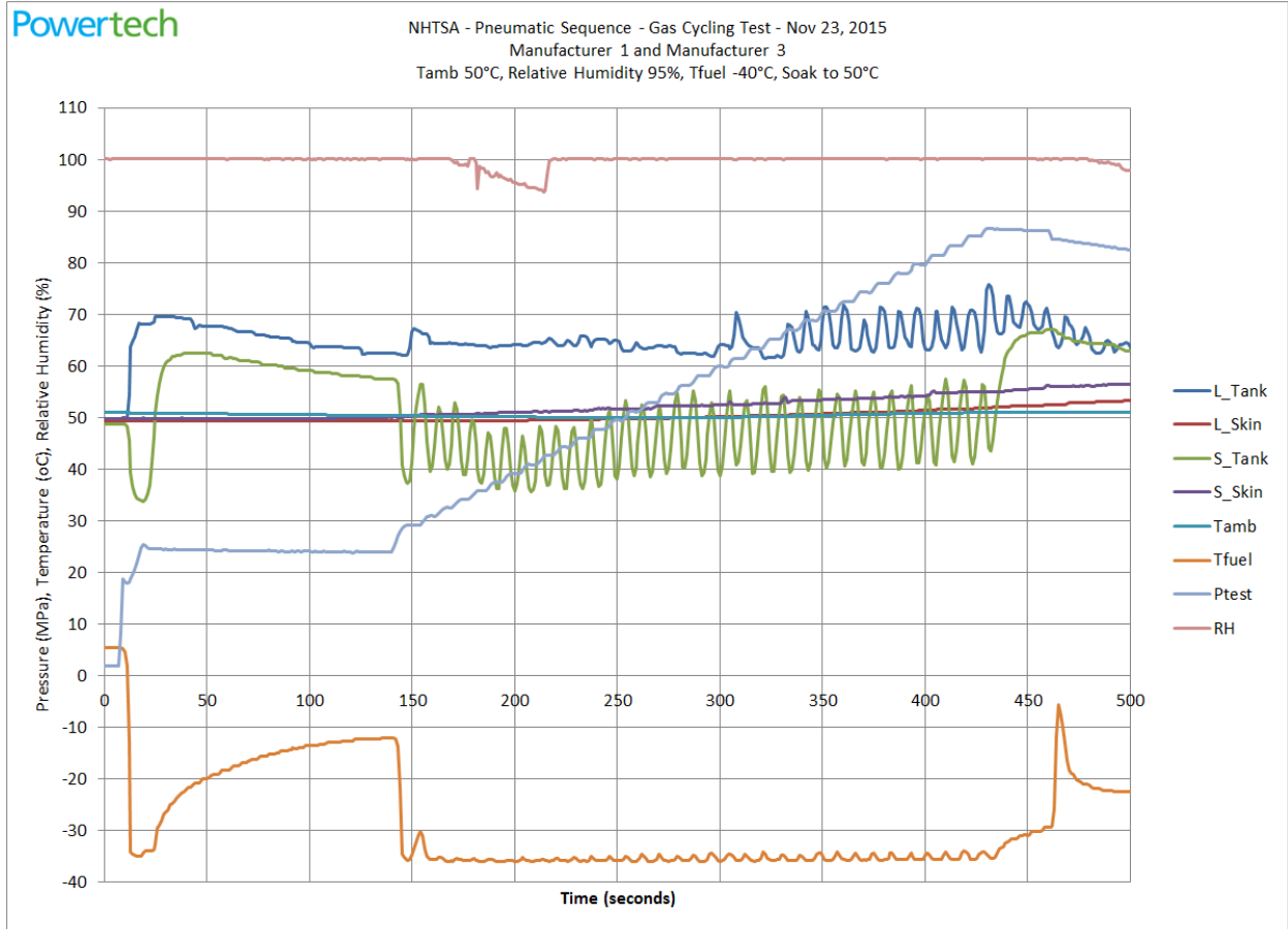
Figure 51. Gas Cycling Test Stage 4 – hot soak cycles, fill profile
