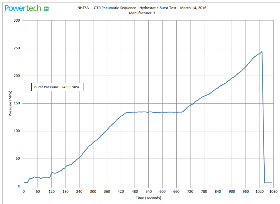
Figure 67. Pneumatic Sequence Burst Test, Container 3-F
