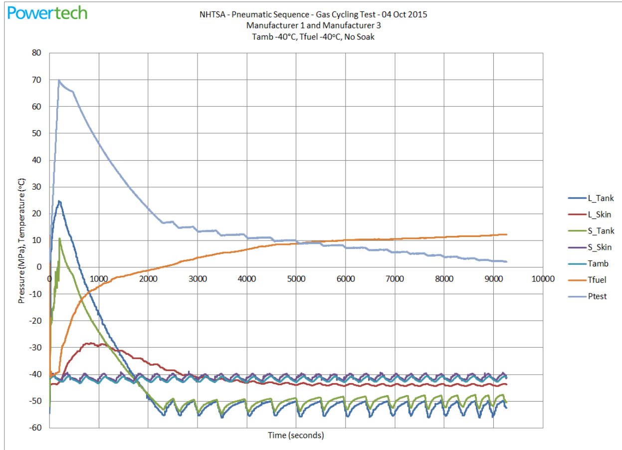
Figure 48. Gas Cycling Test Stage 3 – cold cycles, full cycle
