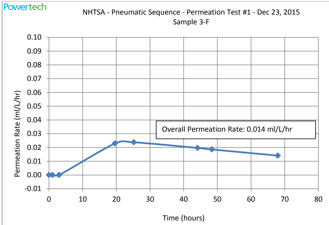
Figure 63. Permeation Test #1, Container 3-F
