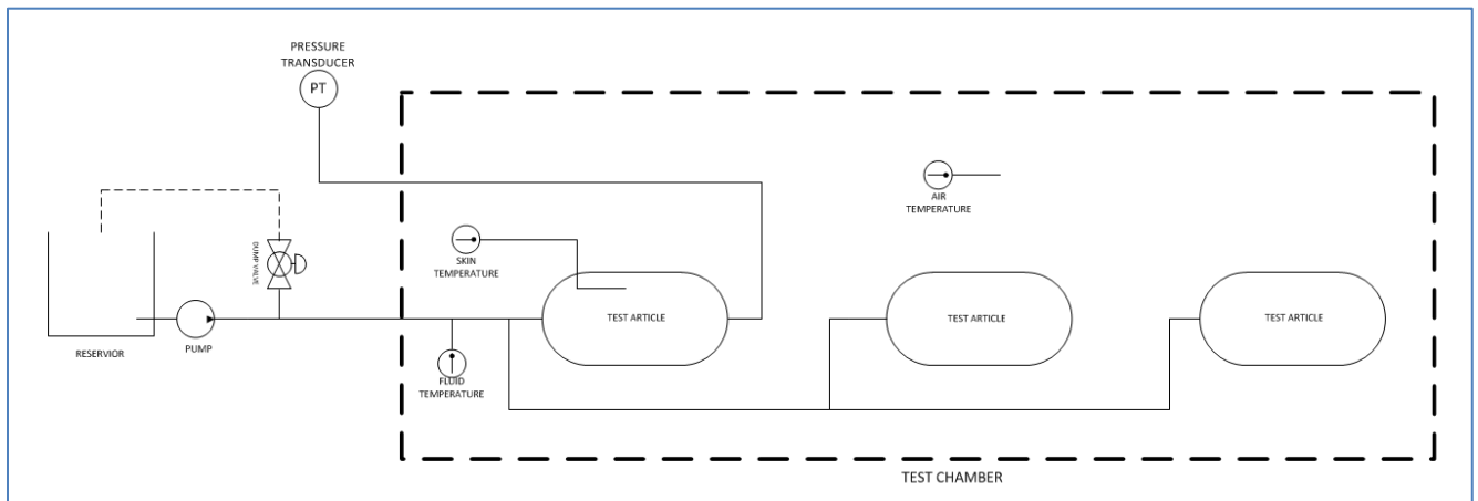
Figure 11. Chemical Exposure and Ambient Temperature Pressure Cycling Test Setup
