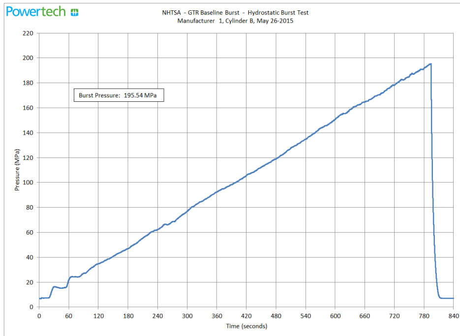
Figure 27. Baseline Burst Pressure Plot of Container 1-B
