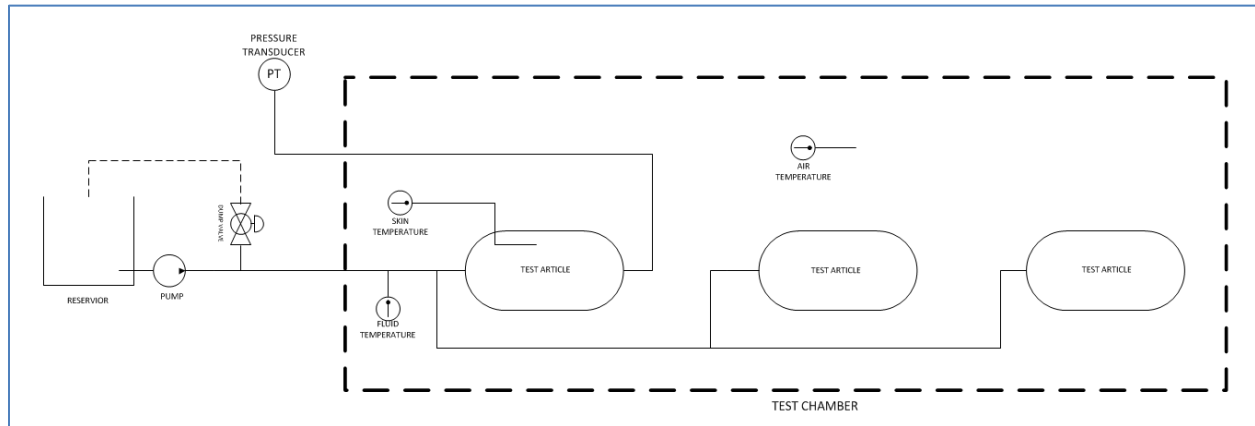
Figure 2. Baseline Initial Pressure Cycling Test Setup
