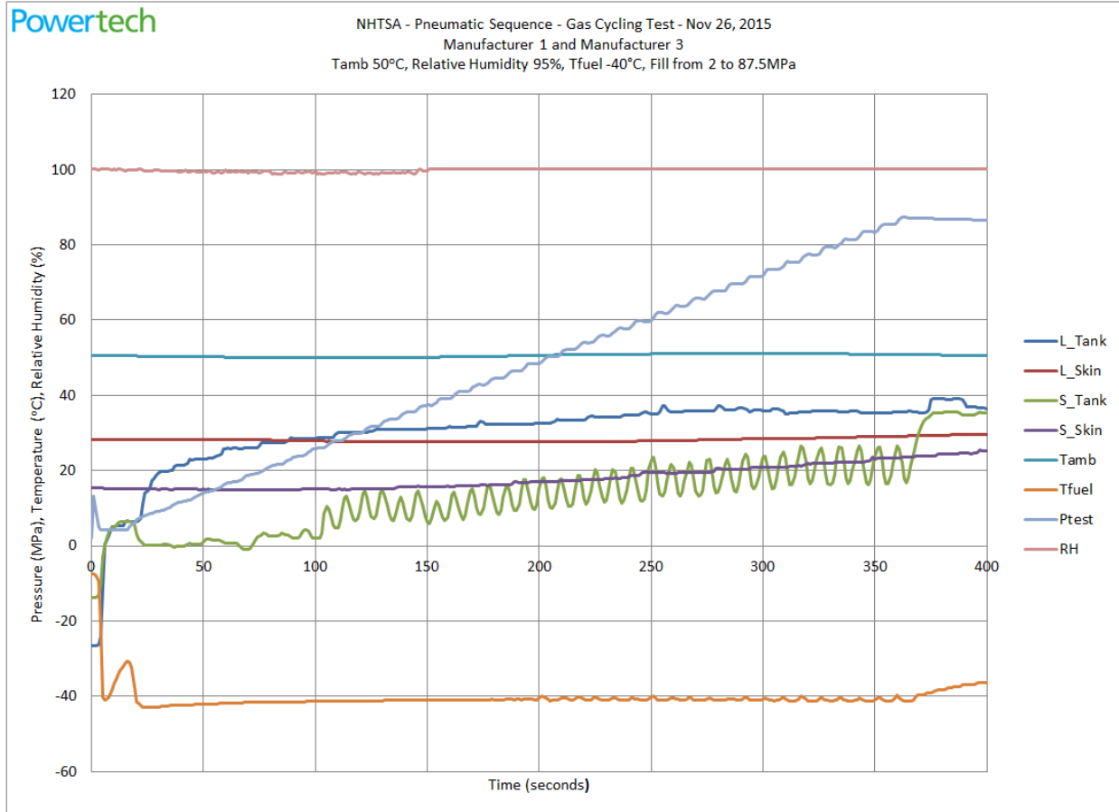
Figure 53. Gas Cycling Test Stage 5 – hot cycles, fill profile
