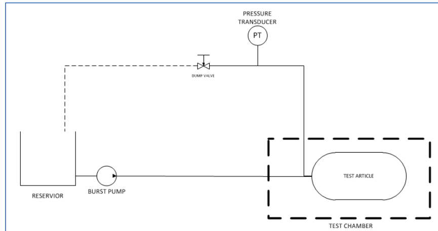
Figure 1. Baseline Burst Test Setup
