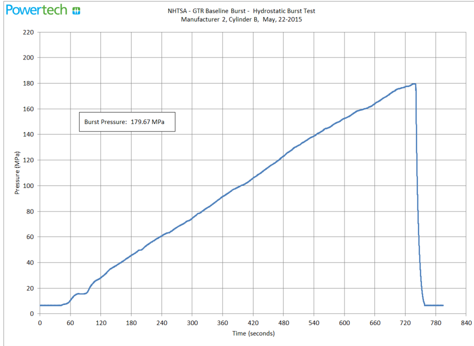
Figure 30. Baseline Burst Pressure Plot of Container 2-B
