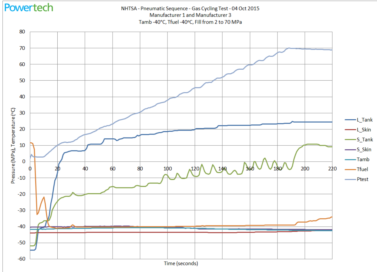
Figure 49. Gas Cycling Test Stage 3 – cold cycles, fill profile
