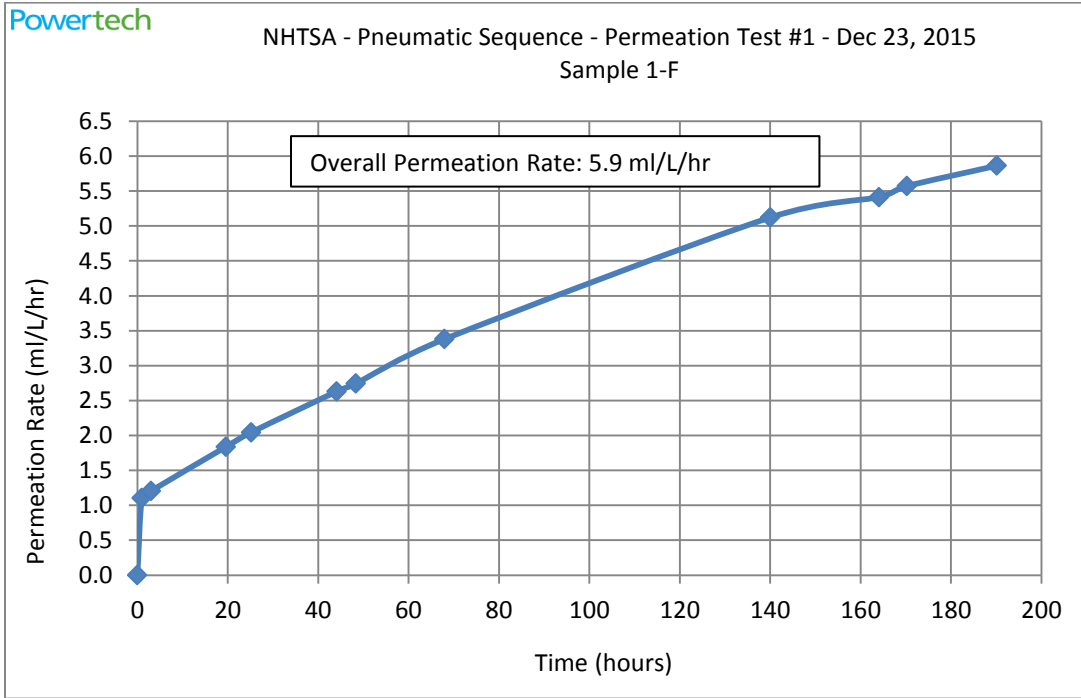
Figure 62. Permeation Test #1 – Container 1-F
