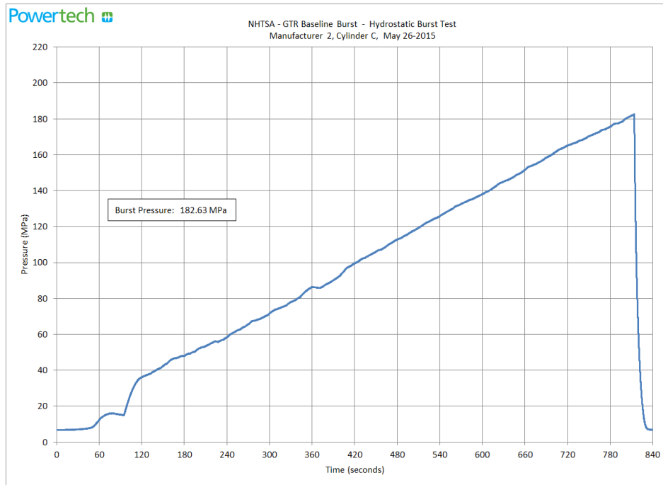
Figure 31. Baseline Burst Pressure Plot of Container 2-C
