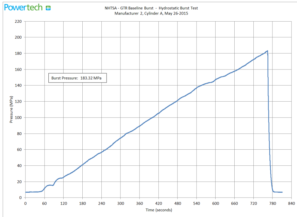
Figure 29. Baseline Burst Pressure Plot of Container 2-A
