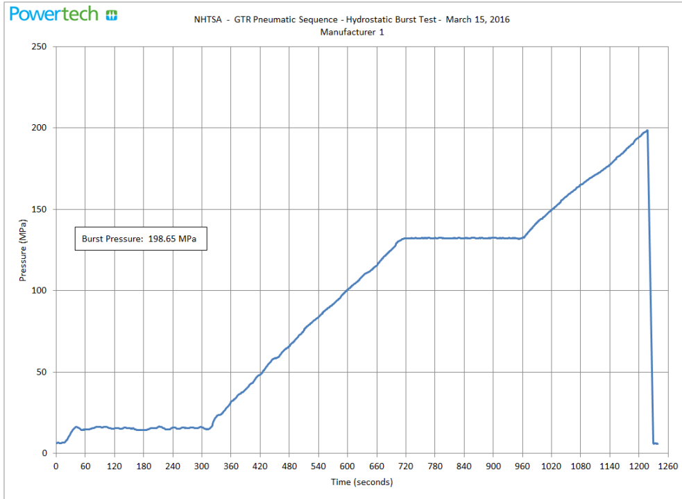
Figure 66. Pneumatic Sequence Burst Test, Container 1-F
