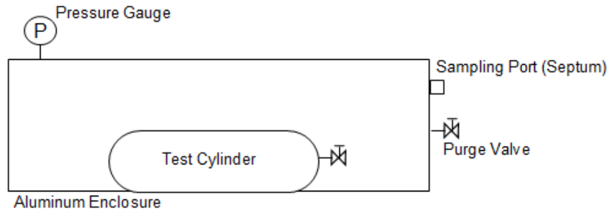
Figure 22. Permeation Test Setup
