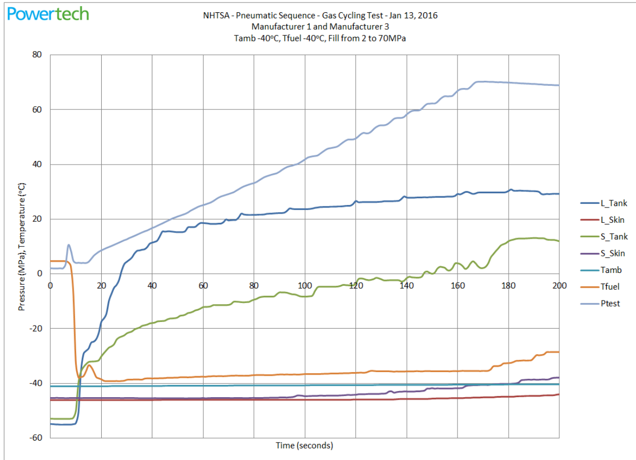
Figure 59. Gas Cycling Test Stage 9 – cold cycles, fill profile
