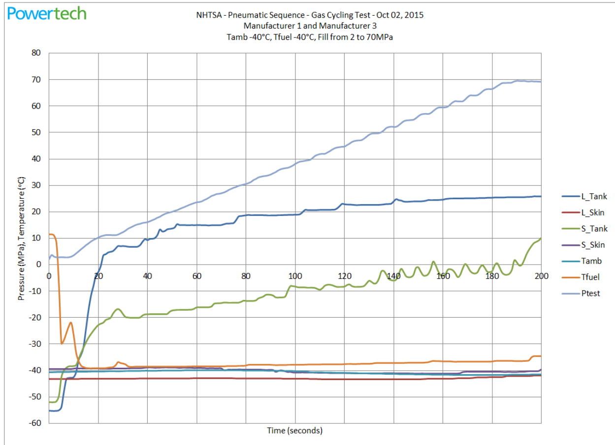
Figure 47. Gas Cycling Test Stage 2 – cold soak cycles with -40°C fuel delivery temperature, fill profile
