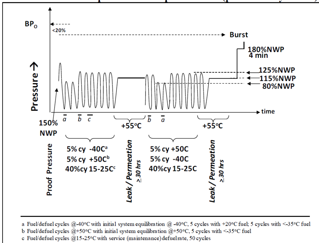
Figure 19. GTR pneumatic sequence diagram (copied from SAE J2579)
