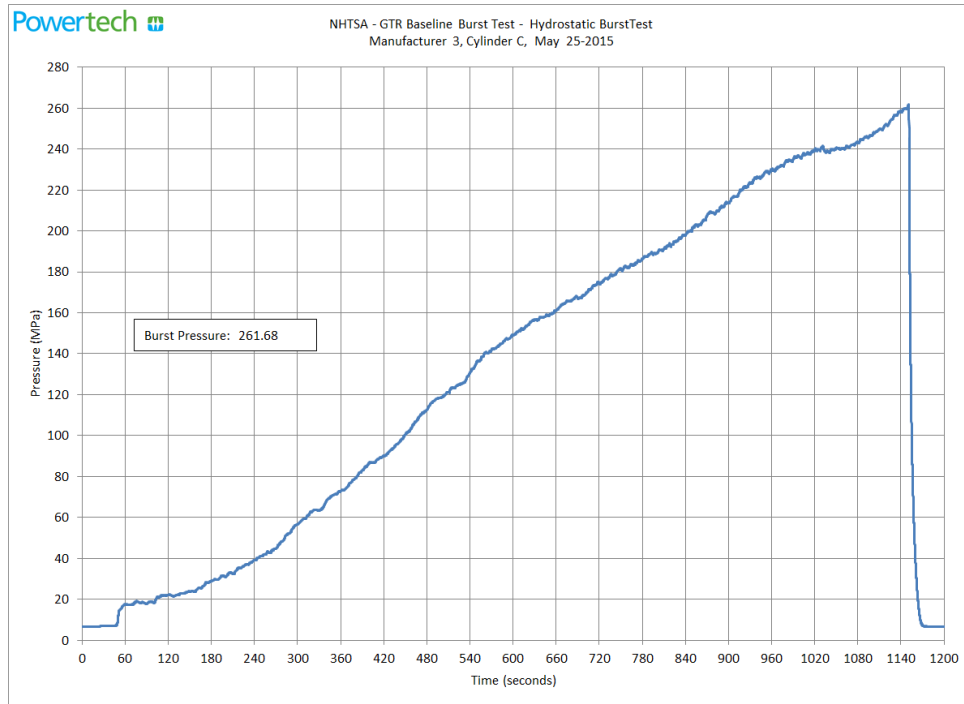
Figure 34. Baseline Burst Pressure Plot of Container 3-C
