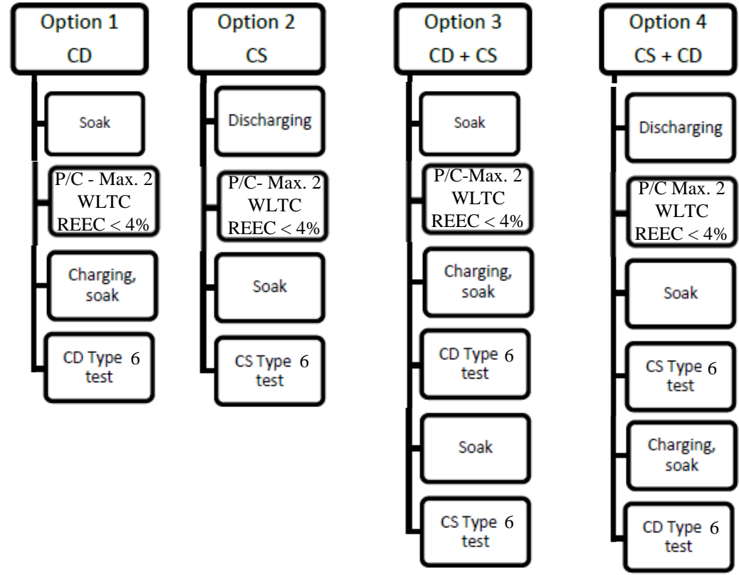
Possible test sequences in the case of OVC-HEV testing
